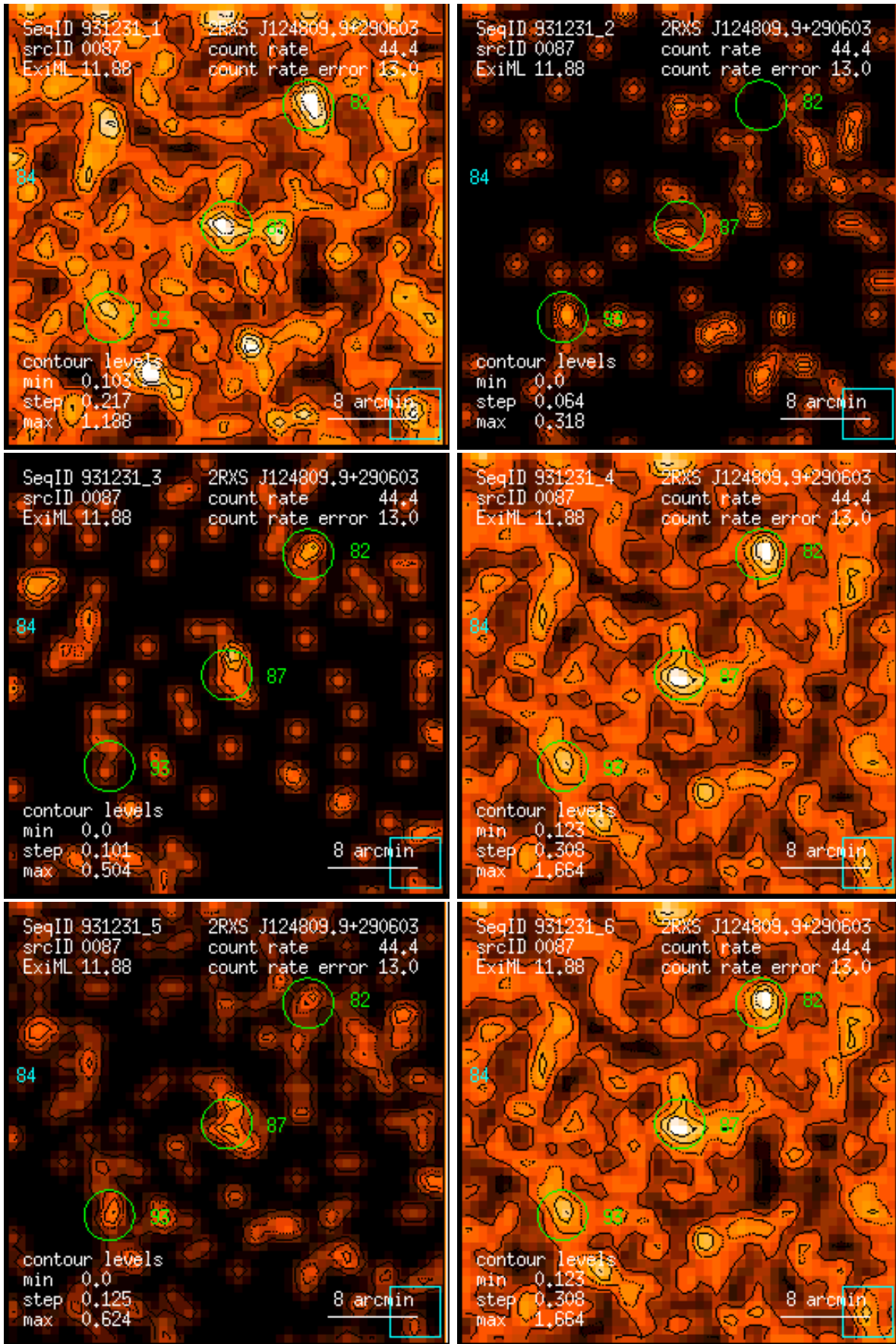
Figure 87: RASS 931231: detection 0087: band rate images, Gaussian filter: (1) PSPC channels 11 – 41, (2) 52 – 90, (3) 91 – 201, (4) 11 – 235, (5) 52 – 201, (6) 11 – 201. Broad band rates in counts/ks. Band rate contour levels in counts/ks/arcmin 2 .
