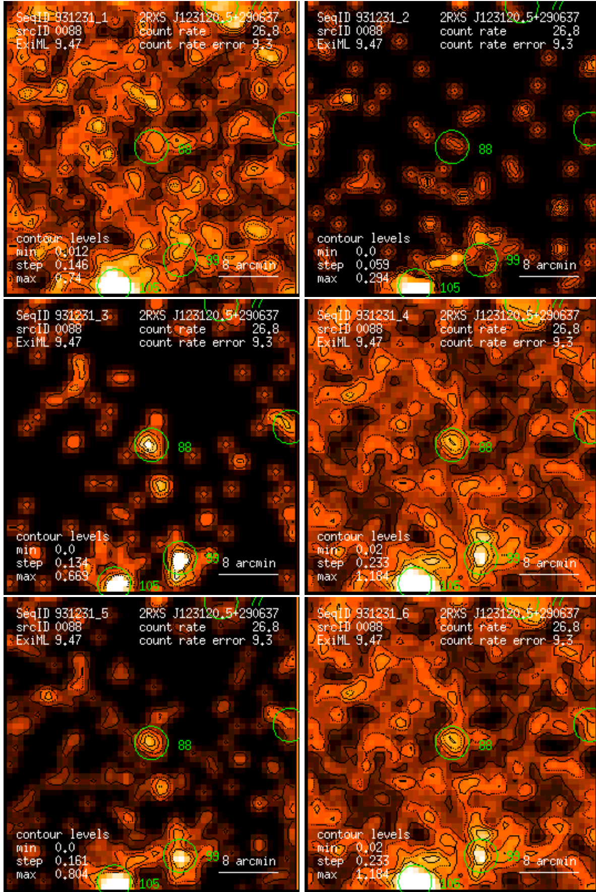
Figure 88: RASS 931231: detection 0088: band rate images, Gaussian filter: (1) PSPC channels 11 – 41, (2) 52 – 90, (3) 91 – 201, (4) 11 – 235, (5) 52 – 201, (6) 11 – 201. Broad band rates in counts/ks. Band rate contour levels in counts/ks/arcmin 2 .
