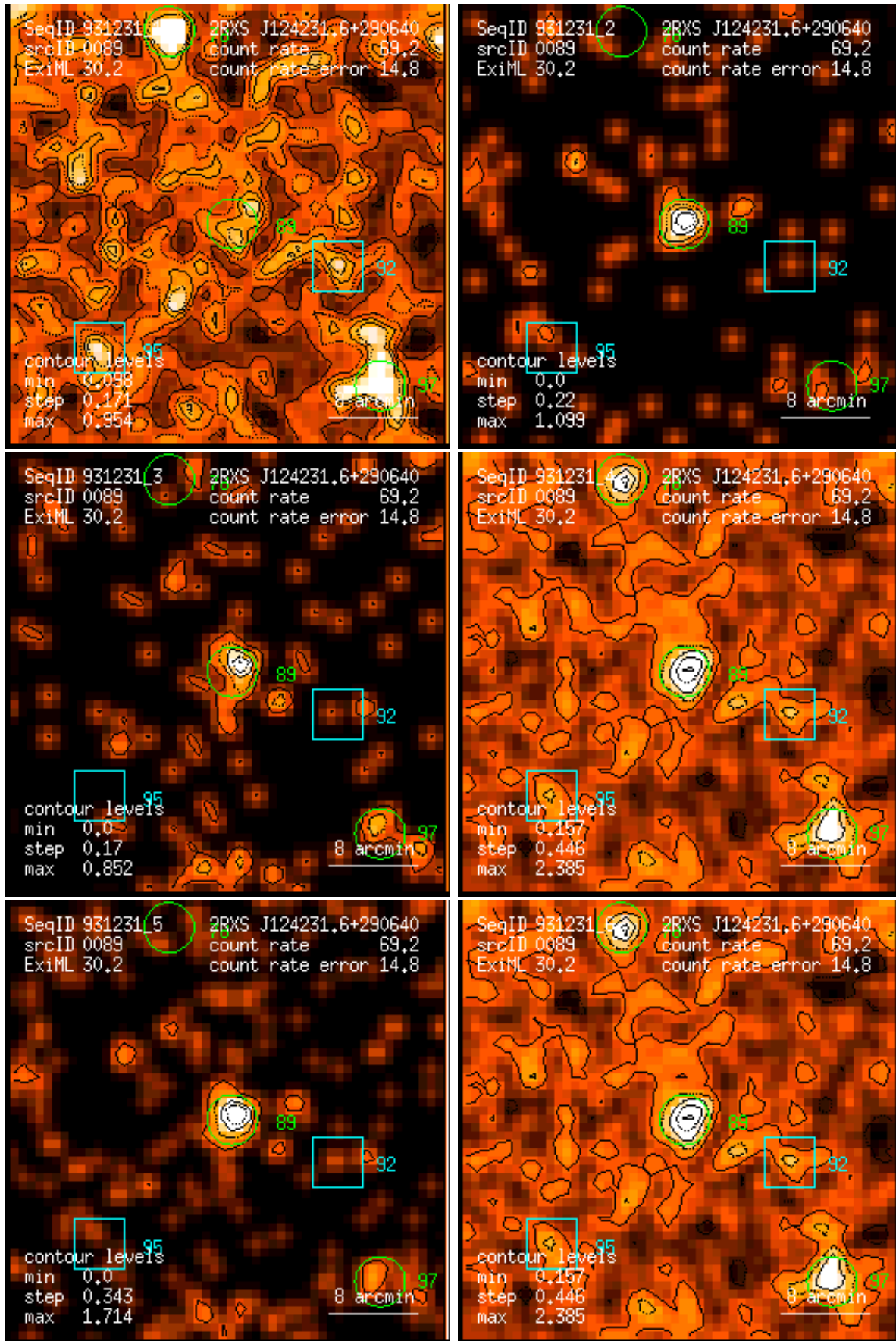
Figure 89: RASS 931231: detection 0089: band rate images, Gaussian filter: (1) PSPC channels 11 – 41, (2) 52 – 90, (3) 91 – 201, (4) 11 – 235, (5) 52 – 201, (6) 11 – 201. Broad band rates in counts/ks. Band rate contour levels in counts/ks/arcmin 2 .
