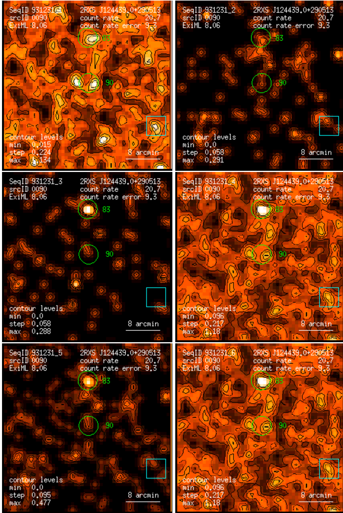
Figure 90: RASS 931231: detection 0090: band rate images, Gaussian filter: (1) PSPC channels 11 – 41, (2) 52 – 90, (3) 91 – 201, (4) 11 – 235, (5) 52 – 201, (6) 11 – 201. Broad band rates in counts/ks. Band rate contour levels in counts/ks/arcmin 2 .
