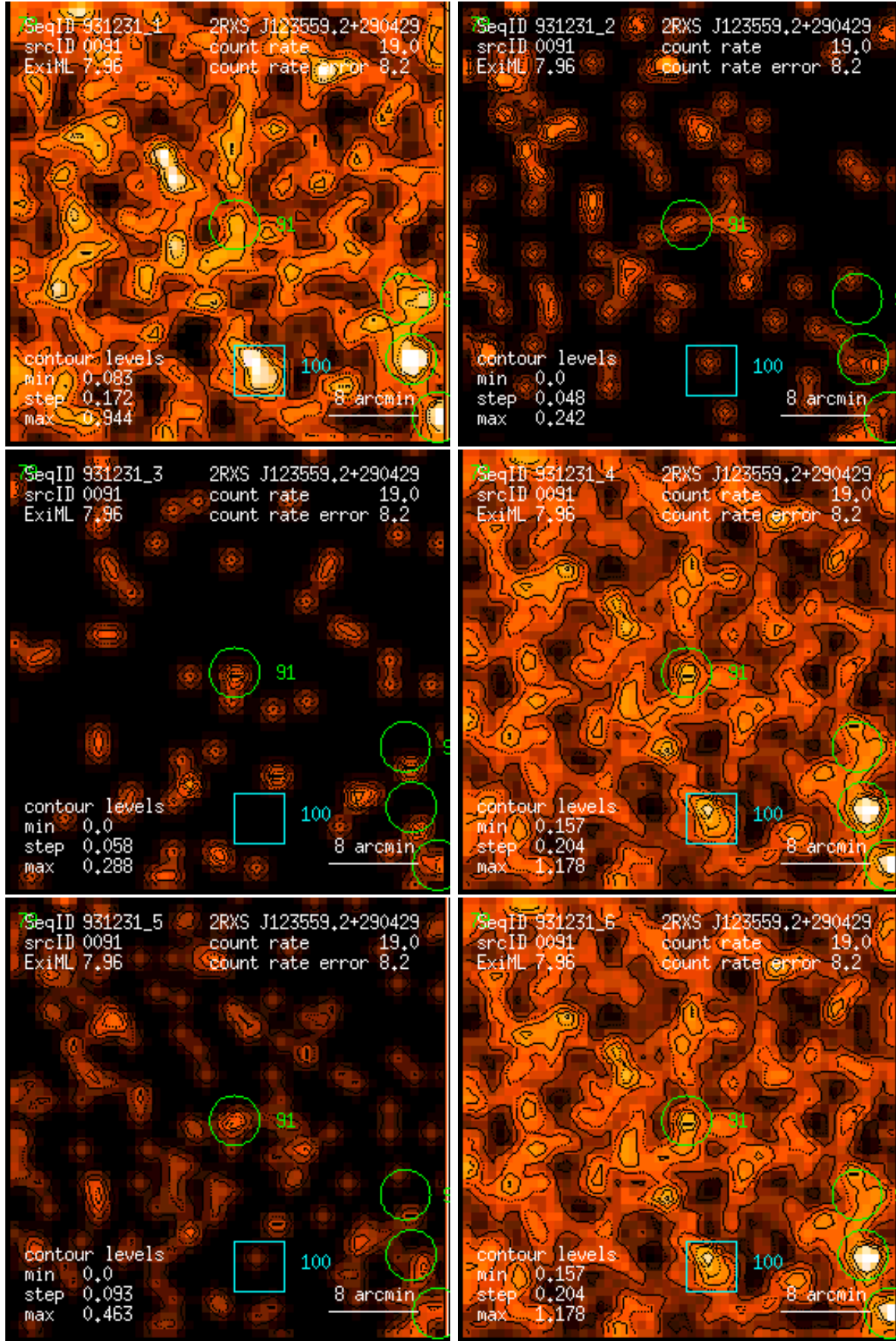
Figure 91: RASS 931231: detection 0091: band rate images, Gaussian filter: (1) PSPC channels 11 – 41, (2) 52 – 90, (3) 91 – 201, (4) 11 – 235, (5) 52 – 201, (6) 11 – 201. Broad band rates in counts/ks. Band rate contour levels in counts/ks/arcmin 2 .
