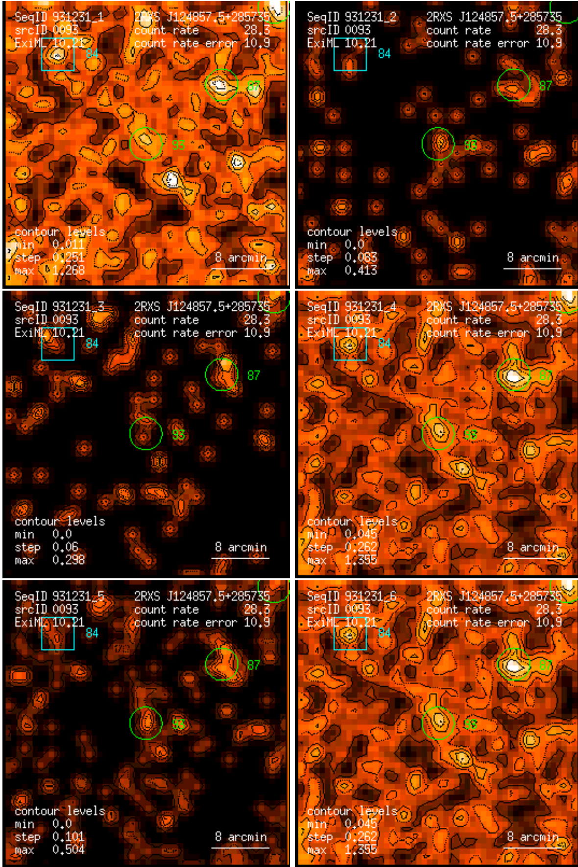
Figure 93: RASS 931231: detection 0093: band rate images, Gaussian filter: (1) PSPC channels 11 – 41, (2) 52 – 90, (3) 91 – 201, (4) 11 – 235, (5) 52 – 201, (6) 11 – 201. Broad band rates in counts/ks. Band rate contour levels in counts/ks/arcmin 2 .
