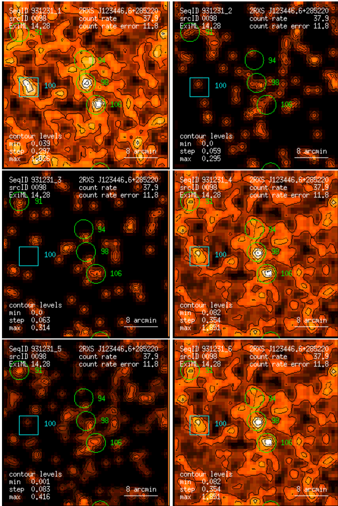
Figure 98: RASS 931231: detection 0098: band rate images, Gaussian filter: (1) PSPC channels 11 – 41, (2) 52 – 90, (3) 91 – 201, (4) 11 – 235, (5) 52 – 201, (6) 11 – 201. Broad band rates in counts/ks. Band rate contour levels in counts/ks/arcmin 2 .
