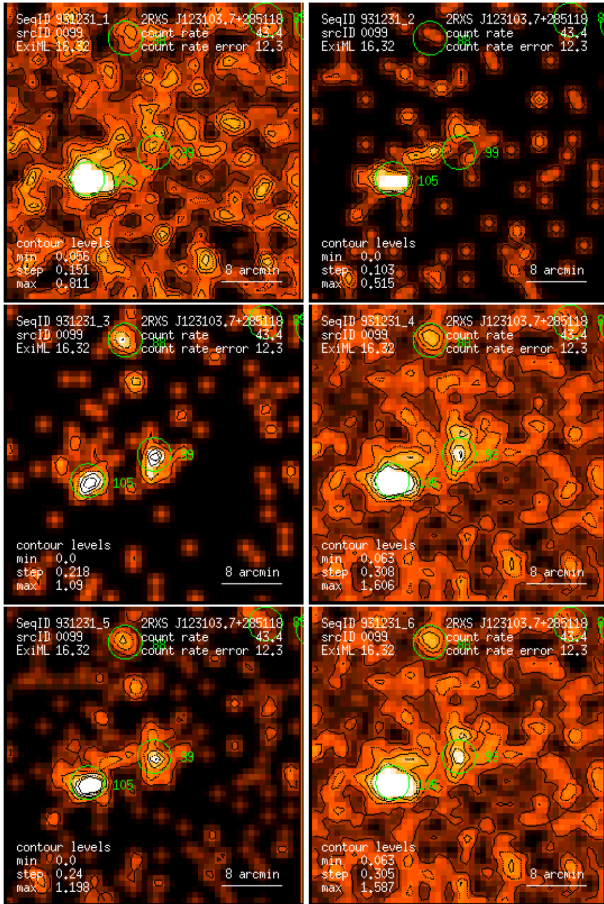
Figure 99: RASS 931231: detection 0099: band rate images, Gaussian filter: (1) PSPC channels 11 – 41, (2) 52 – 90, (3) 91 – 201, (4) 11 – 235, (5) 52 – 201, (6) 11 – 201. Broad band rates in counts/ks. Band rate contour levels in counts/ks/arcmin 2 .
