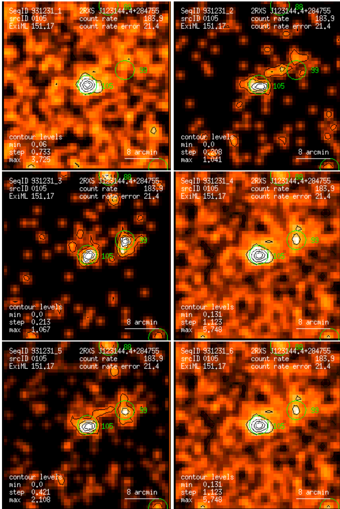
Figure 105: RASS 931231: detection 0105: band rate images, Gaussian filter: (1) PSPC channels 11 – 41, (2) 52 – 90, (3) 91 – 201, (4) 11 – 235, (5) 52 – 201, (6) 11 – 201. Broad band rates in counts/ks. Band rate contour levels in counts/ks/arcmin 2 .
