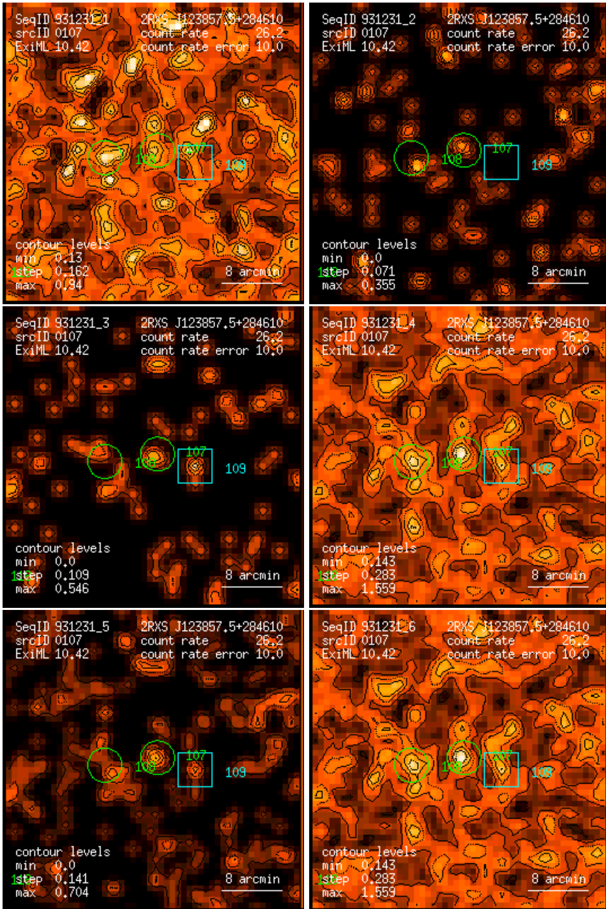
Figure 107: RASS 931231: detection 0107: band rate images, Gaussian filter: (1) PSPC channels 11 – 41, (2) 52 – 90, (3) 91 – 201, (4) 11 – 235, (5) 52 – 201, (6) 11 – 201. Broad band rates in counts/ks. Band rate contour levels in counts/ks/arcmin 2 .
