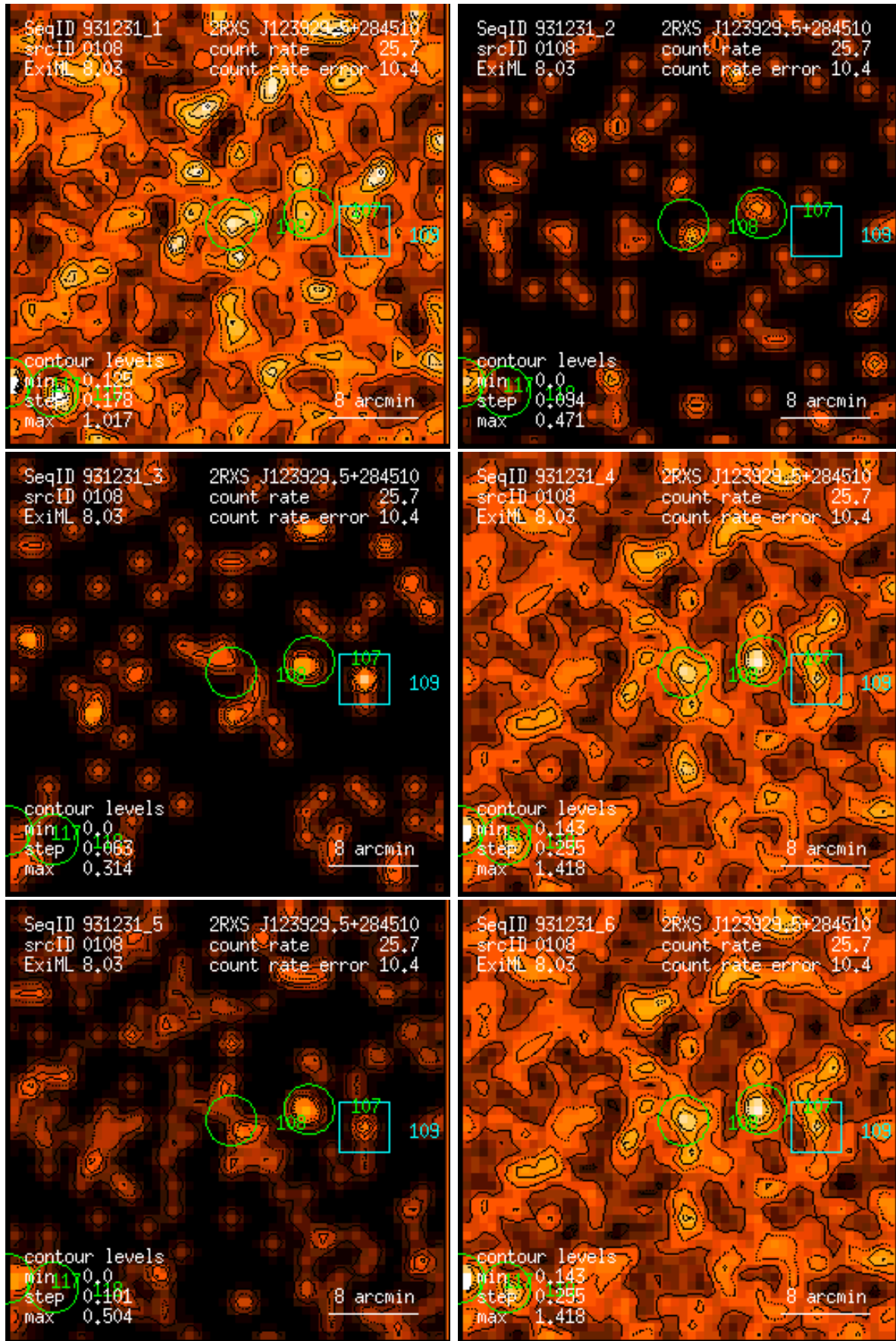
Figure 108: RASS 931231: detection 0108: band rate images, Gaussian filter: (1) PSPC channels 11 – 41, (2) 52 – 90, (3) 91 – 201, (4) 11 – 235, (5) 52 – 201, (6) 11 – 201. Broad band rates in counts/ks. Band rate contour levels in counts/ks/arcmin 2 .
