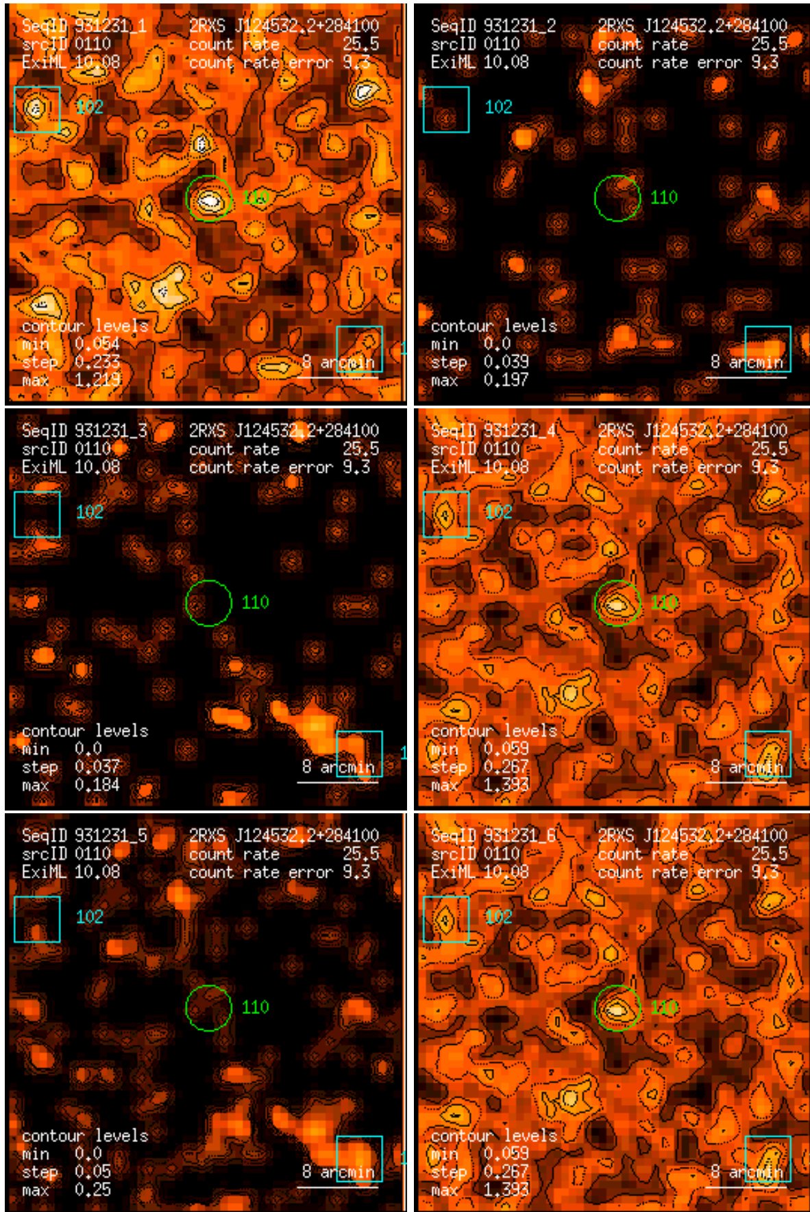
Figure 110: RASS 931231: detection 0110: band rate images, Gaussian filter: (1) PSPC channels 11 – 41, (2) 52 – 90, (3) 91 – 201, (4) 11 – 235, (5) 52 – 201, (6) 11 – 201. Broad band rates in counts/ks. Band rate contour levels in counts/ks/arcmin 2 .
