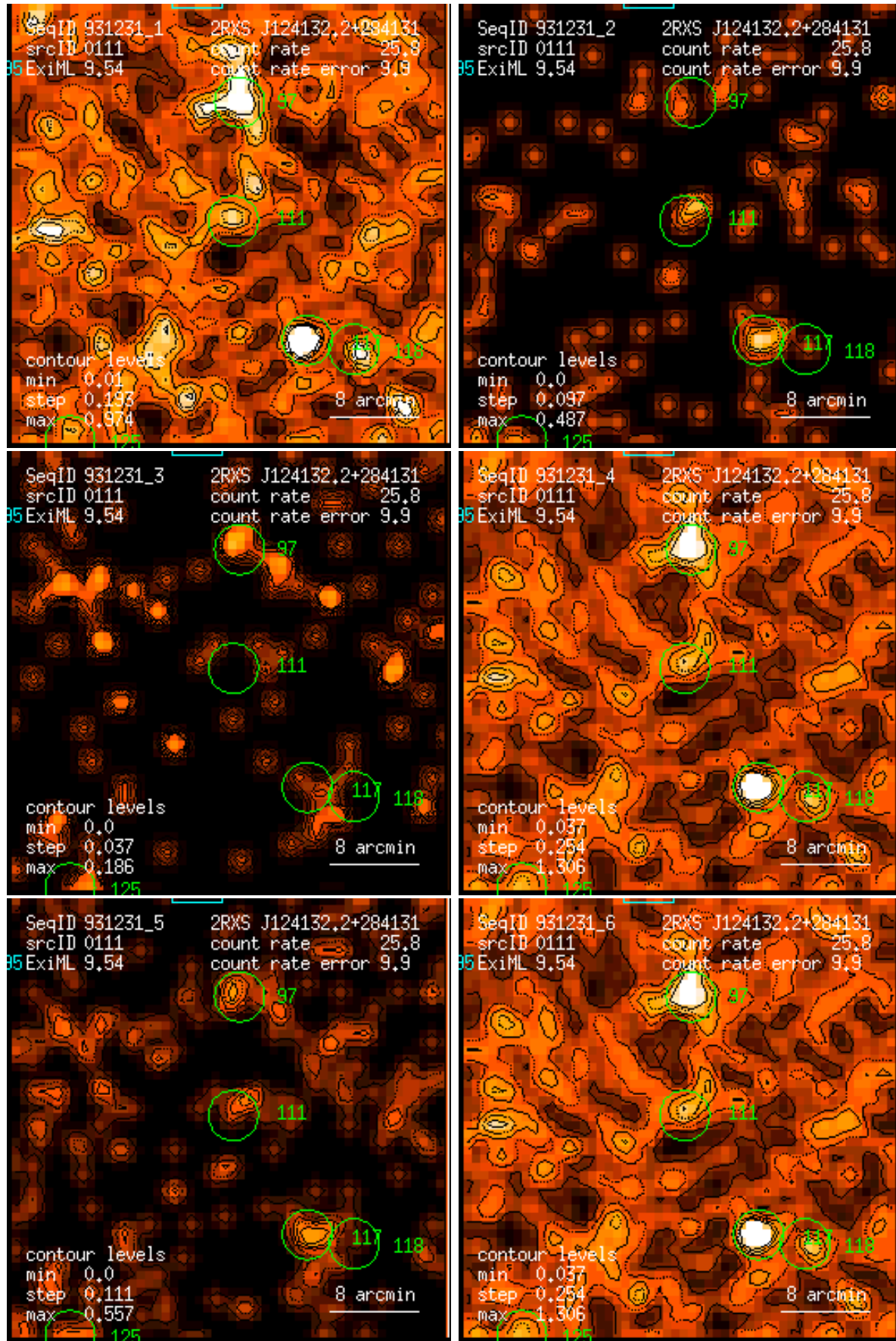
Figure 111: RASS 931231: detection 0111: band rate images, Gaussian filter: (1) PSPC channels 11 – 41, (2) 52 – 90, (3) 91 – 201, (4) 11 – 235, (5) 52 – 201, (6) 11 – 201. Broad band rates in counts/ks. Band rate contour levels in counts/ks/arcmin 2 .
