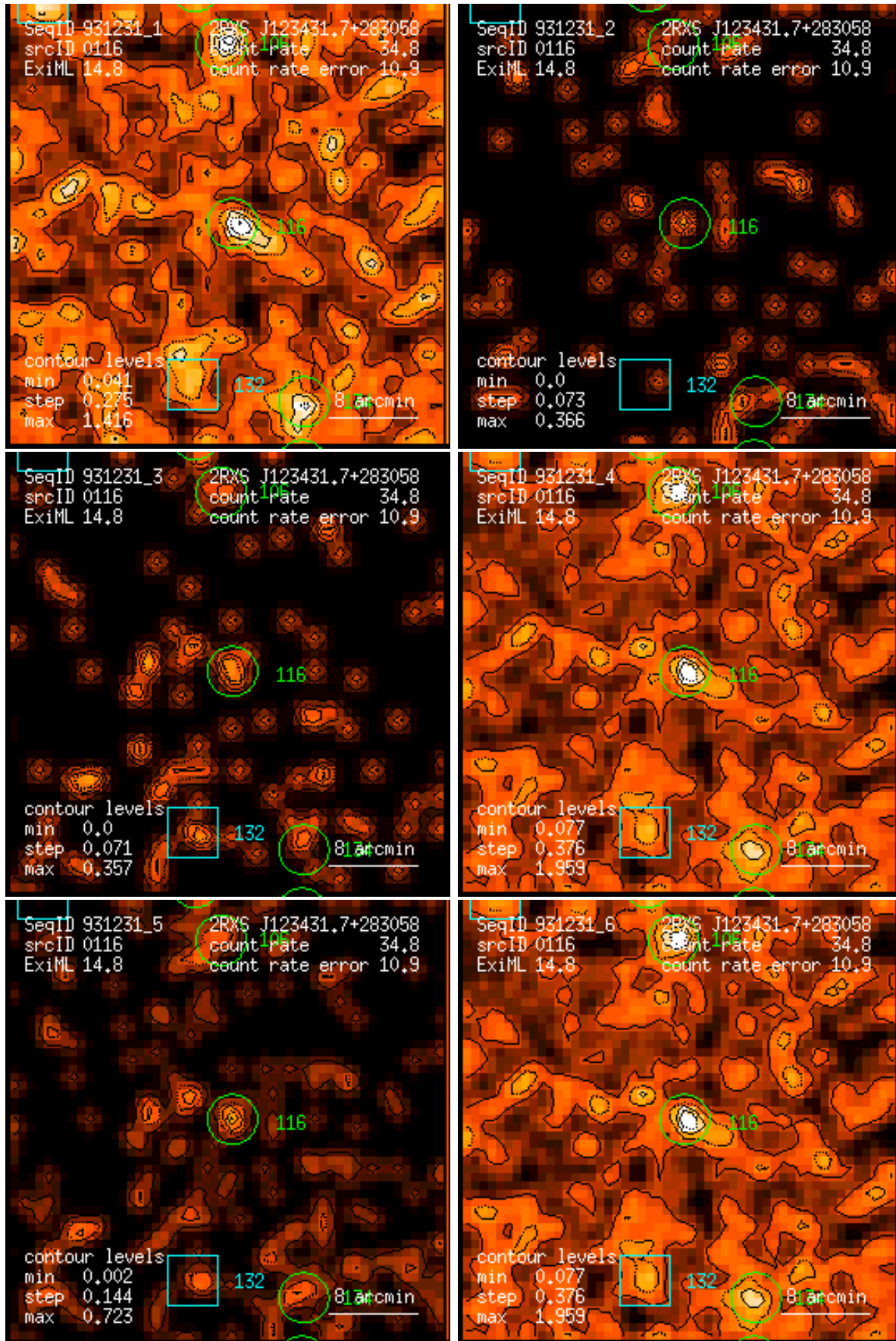
Figure 116: RASS 931231: detection 0116: band rate images, Gaussian filter: (1) PSPC channels 11 – 41, (2) 52 – 90, (3) 91 – 201, (4) 11 – 235, (5) 52 – 201, (6) 11 – 201. Broad band rates in counts/ks. Band rate contour levels in counts/ks/arcmin 2 .
