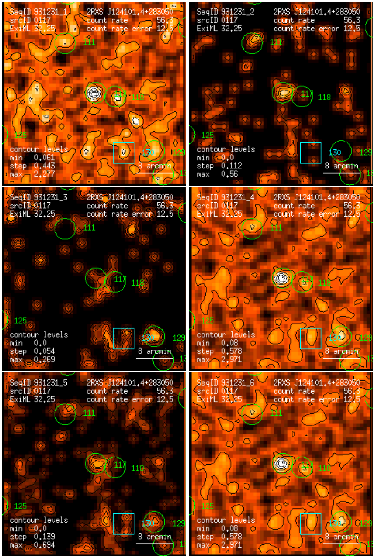
Figure 117: RASS 931231: detection 0117: band rate images, Gaussian filter: (1) PSPC channels 11 – 41, (2) 52 – 90, (3) 91 – 201, (4) 11 – 235, (5) 52 – 201, (6) 11 – 201. Broad band rates in counts/ks. Band rate contour levels in counts/ks/arcmin 2 .
