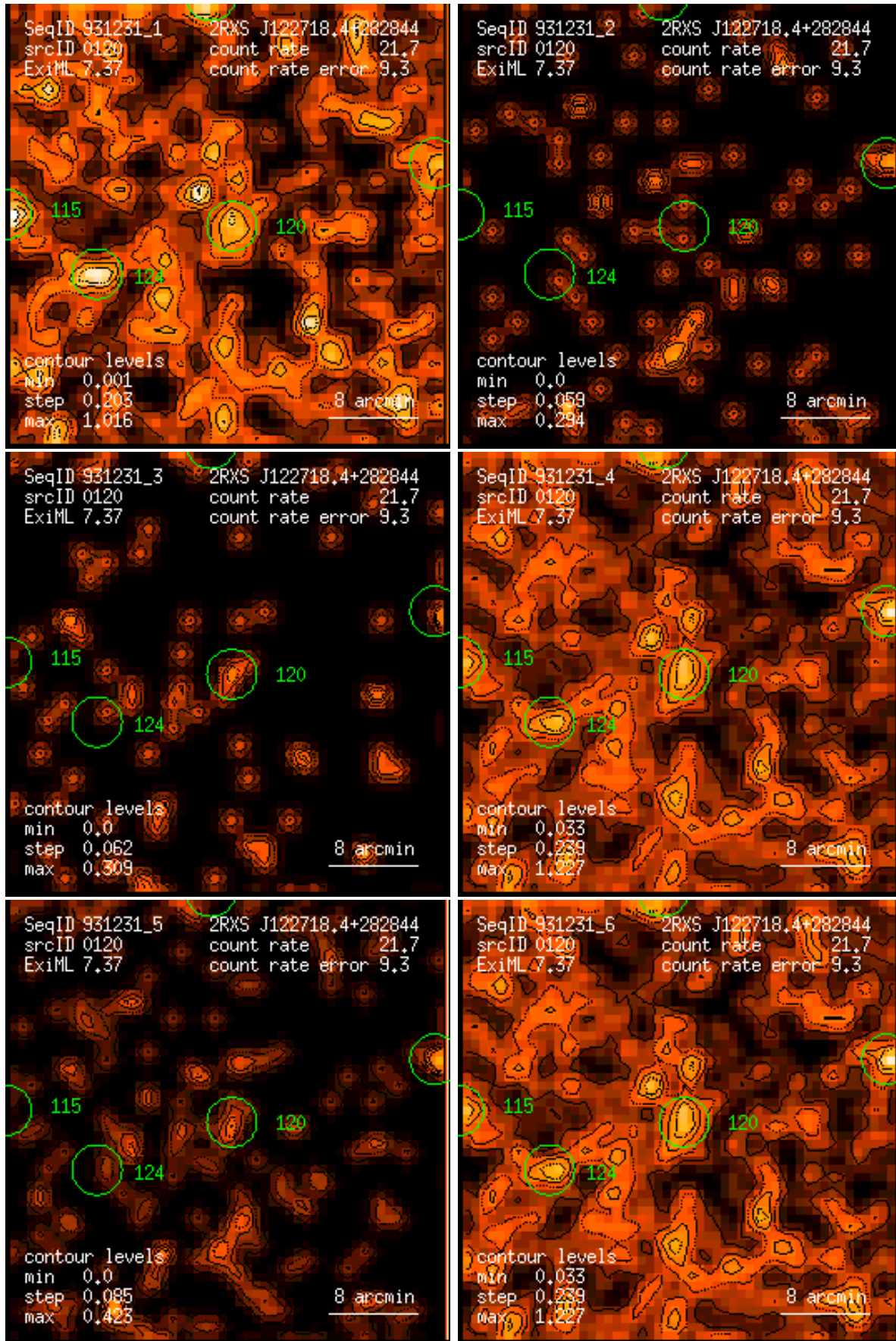
Figure 120: RASS 931231: detection 0120: band rate images, Gaussian filter: (1) PSPC channels 11 – 41, (2) 52 – 90, (3) 91 – 201, (4) 11 – 235, (5) 52 – 201, (6) 11 – 201. Broad band rates in counts/ks. Band rate contour levels in counts/ks/arcmin 2 .
