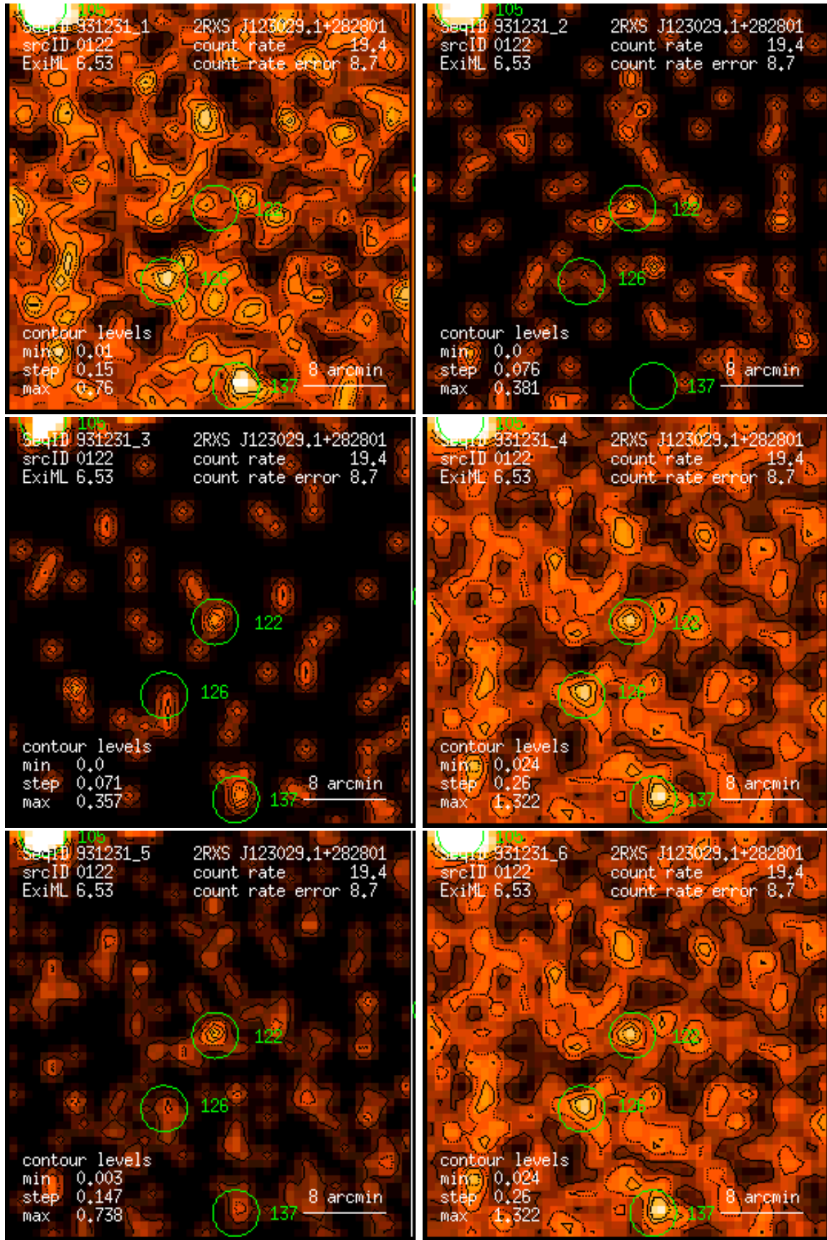
Figure 122: RASS 931231: detection 0122: band rate images, Gaussian filter: (1) PSPC channels 11 – 41, (2) 52 – 90, (3) 91 – 201, (4) 11 – 235, (5) 52 – 201, (6) 11 – 201. Broad band rates in counts/ks. Band rate contour levels in counts/ks/arcmin 2 .
