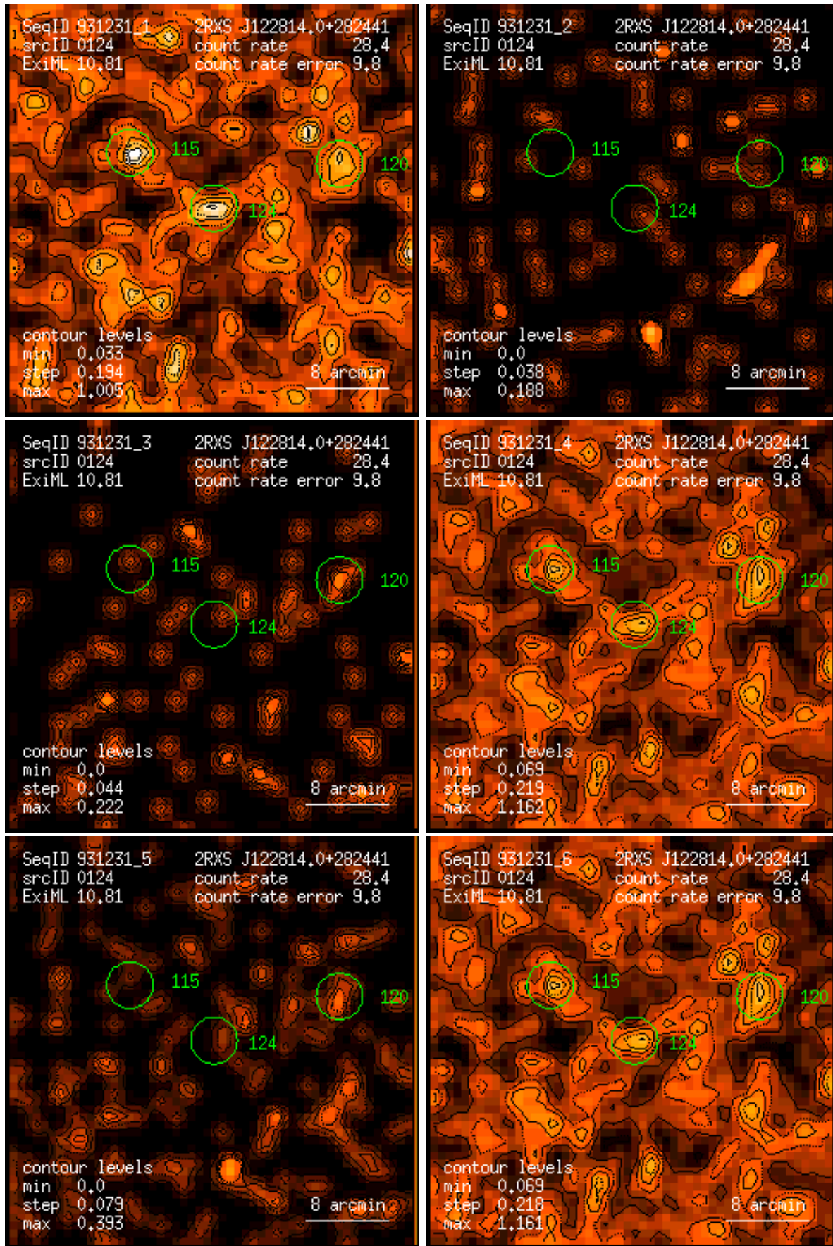
Figure 124: RASS 931231: detection 0124: band rate images, Gaussian filter: (1) PSPPC channels 11 – 41, (2) 52 – 90, (3) 91 – 201, (4) 11 – 235, (5) 52 – 201, (6) 11 – 201. Broad band rates in counts/ks. Band rate contour levels in counts/ks/arcmin 2 .
