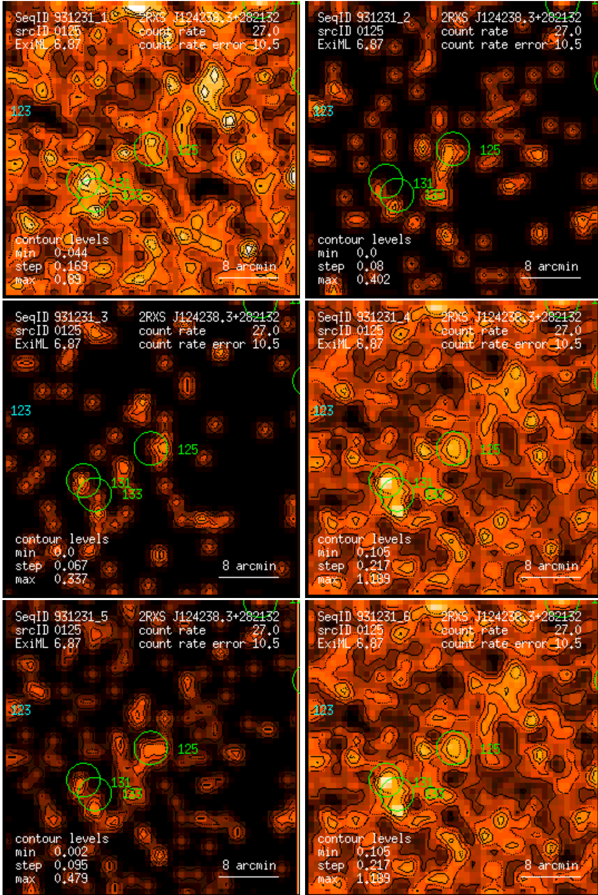
Figure 125: RASS 931231: detection 0125: band rate images, Gaussian filter: (1) PSPC channels 11 – 41, (2) 52 – 90, (3) 91 – 201, (4) 11 – 235, (5) 52 – 201, (6) 11 – 201. Broad band rates in counts/ks. Band rate contour levels in counts/ks/arcmin 2 .
