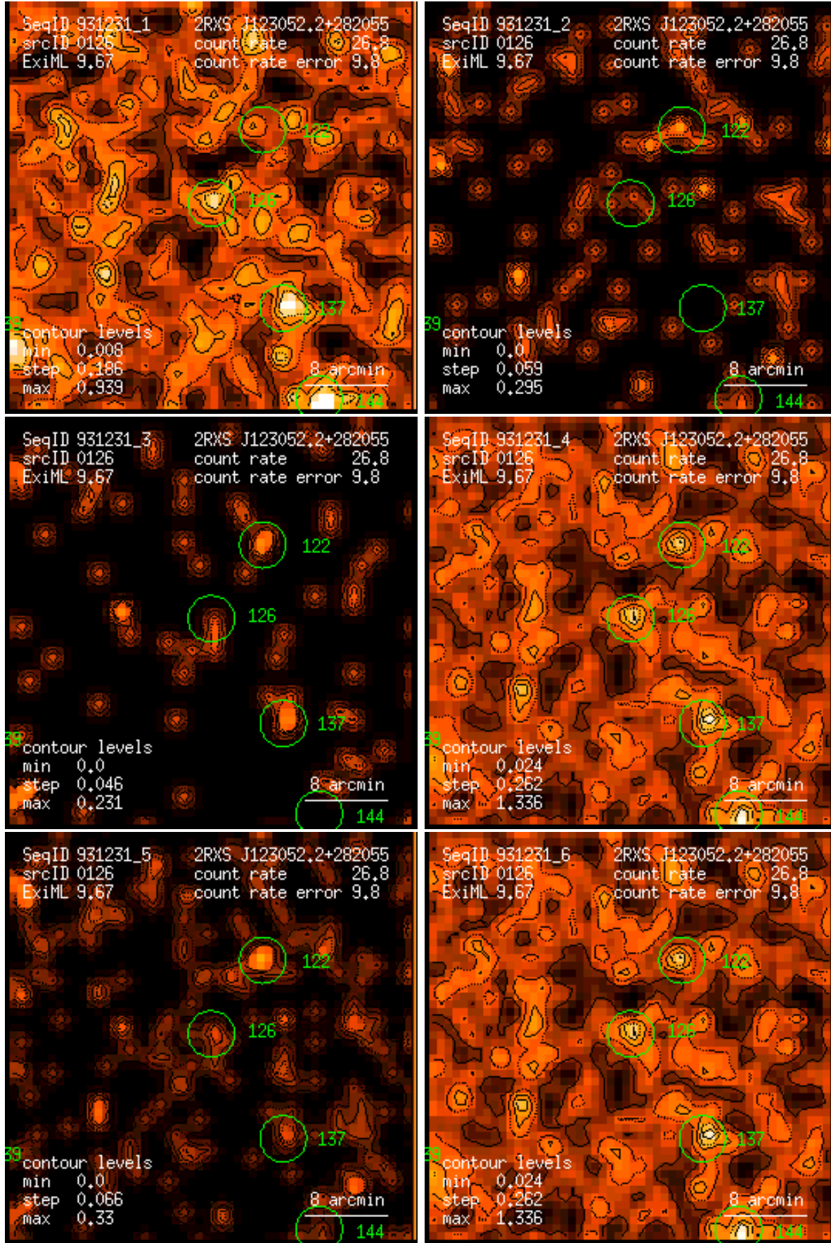
Figure 126: RASS 931231: detection 0126: band rate images, Gaussian filter: (1) PSPC channels 11 – 41, (2) 52 – 90, (3) 91 – 201, (4) 11 – 235, (5) 52 – 201, (6) 11 – 201. Broad band rates in counts/ks. Band rate contour levels in counts/ks/arcmin 2 .
