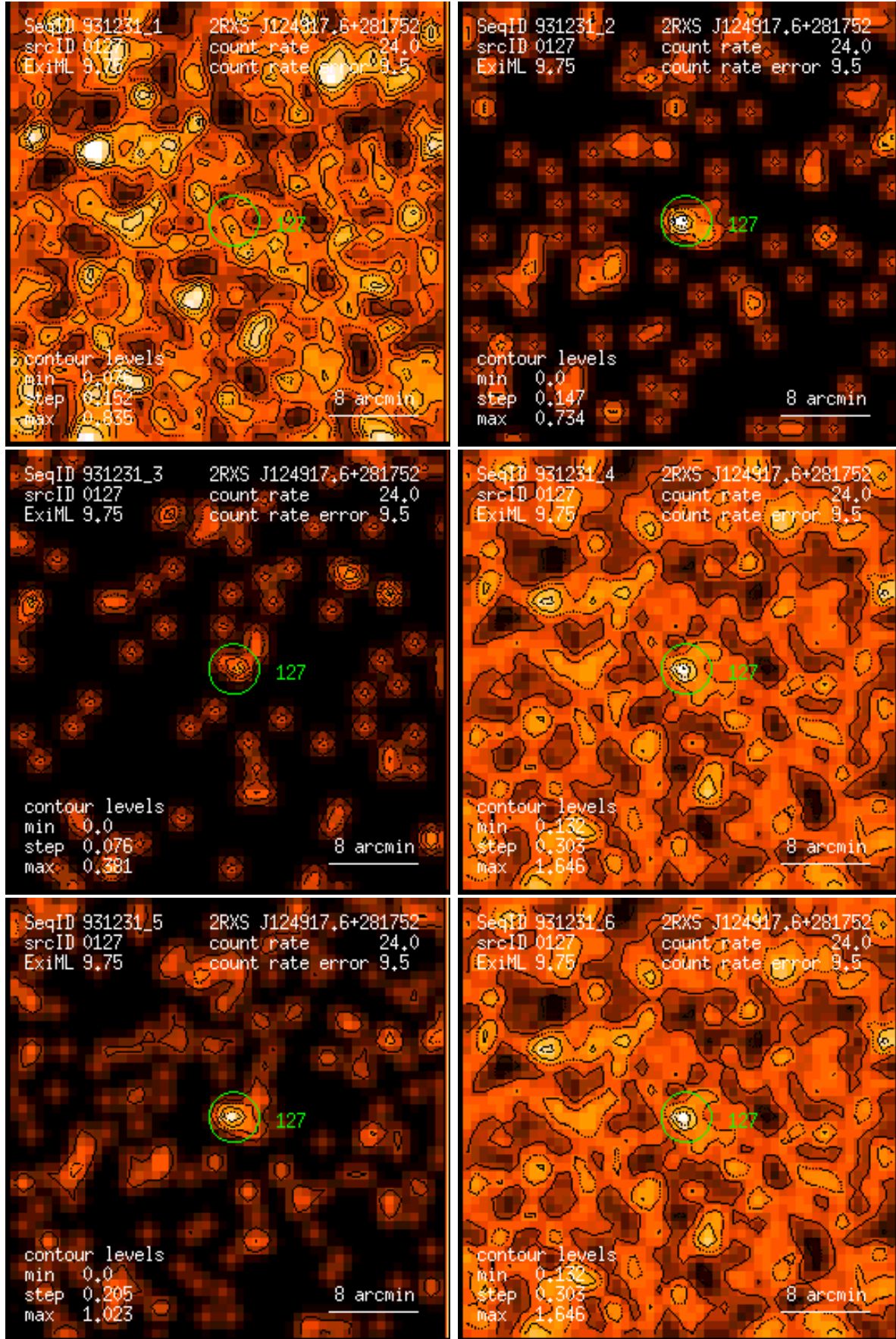
Figure 127: RASS 931231: detection 0127: band rate images, Gaussian filter: (1) PSPC channels 11 – 41, (2) 52 – 90, (3) 91 – 201, (4) 11 – 235, (5) 52 – 201, (6) 11 – 201. Broad band rates in counts/ks. Band rate contour levels in counts/ks/arcmin 2 .
