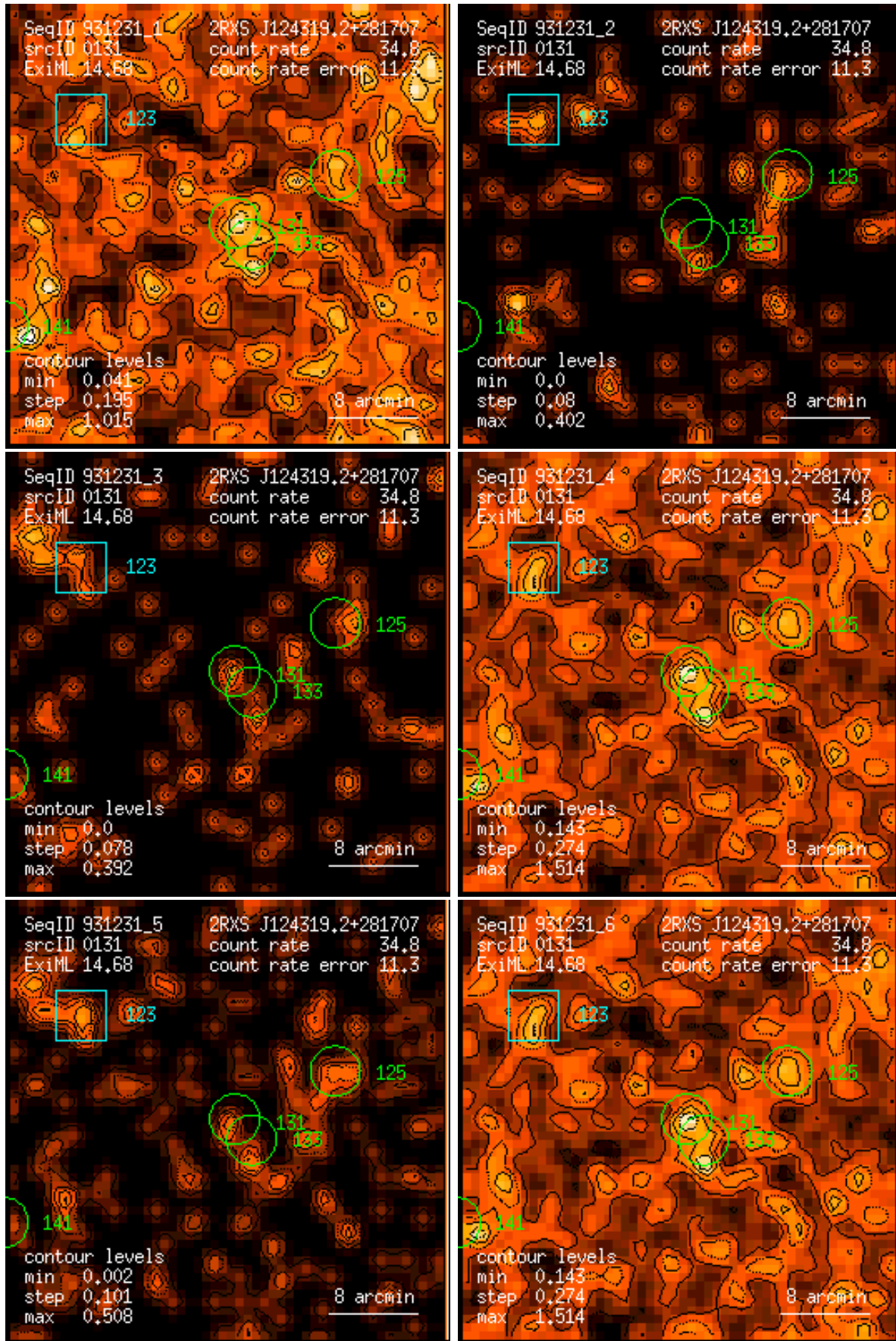
Figure 131: RASS 931231: detection 0131: band rate images, Gaussian filter: (1) PSPC channels 11 – 41, (2) 52 – 90, (3) 91 – 201, (4) 11 – 235, (5) 52 – 201, (6) 11 – 201. Broad band rates in counts/ks. Band rate contour levels in counts/ks/arcmin 2 .
