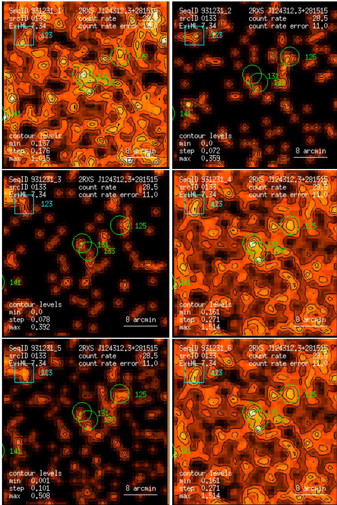
Figure 133: RASS 931231: detection 0133: band rate images, Gaussian filter: (1) PSPC channels 11 – 41, (2) 52 – 90, (3) 91 – 201, (4) 11 – 235, (5) 52 – 201, (6) 11 – 201. Broad band rates in counts/ks. Band rate contour levels in counts/ks/arcmin 2 .
