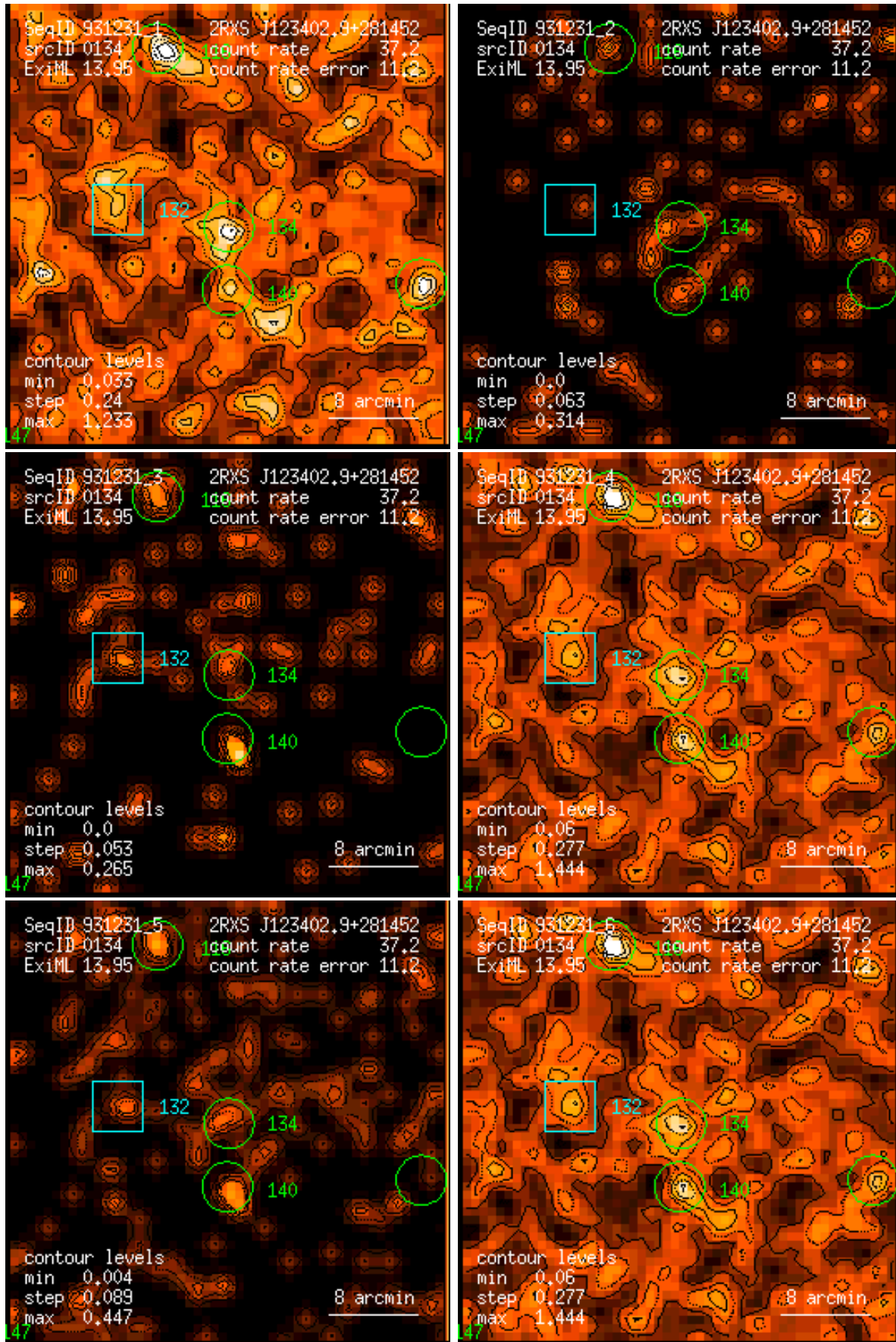
Figure 134: RASS 931231: detection 0134: band rate images, Gaussian filter: (1) PSPC channels 11 – 41, (2) 52 – 90, (3) 91 – 201, (4) 11 – 235, (5) 52 – 201, (6) 11 – 201. Broad band rates in counts/ks. Band rate contour levels in counts/ks/arcmin 2 .
