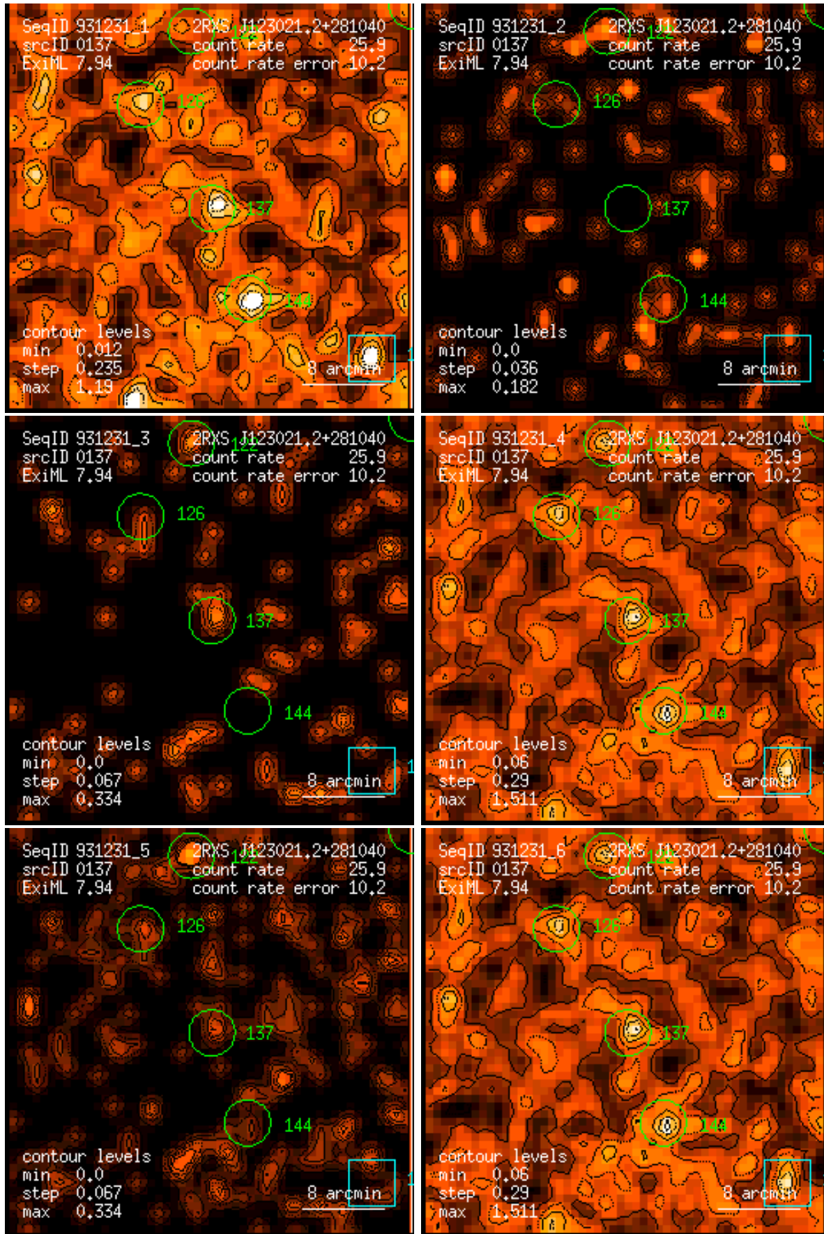
Figure 137: RASS 931231: detection 0137: band rate images, Gaussian filter: (1) PSPC channels 11 – 41, (2) 52 – 90, (3) 91 – 201, (4) 11 – 235, (5) 52 – 201, (6) 11 – 201. Broad band rates in counts/ks. Band rate contour levels in counts/ks/arcmin 2 .
