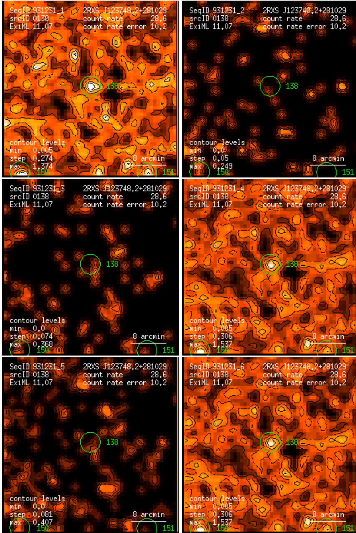
Figure 138: RASS 931231: detection 0138: band rate images, Gaussian filter: (1) PSPC channels 11 – 41, (2) 52 – 90, (3) 91 – 201, (4) 11 – 235, (5) 52 – 201, (6) 11 – 201. Broad band rates in counts/ks. Band rate contour levels in counts/ks/arcmin 2 .
