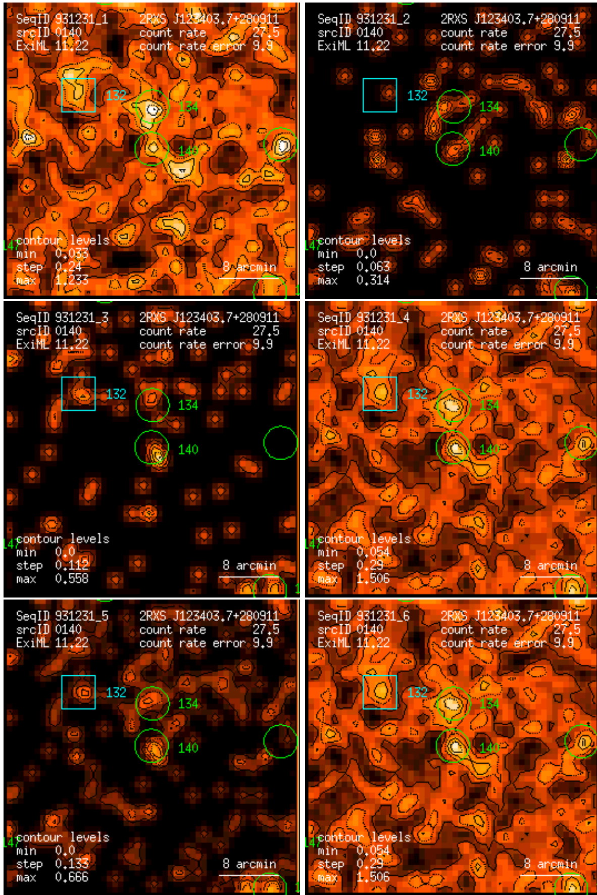
Figure 140: RASS 931231: detection 0140: band rate images, Gaussian filter: (1) PSPC channels 11 – 41, (2) 52 – 90, (3) 91 – 201, (4) 11 – 235, (5) 52 – 201, (6) 11 – 201. Broad band rates in counts/ks. Band rate contour levels in counts/ks/arcmin 2 .
