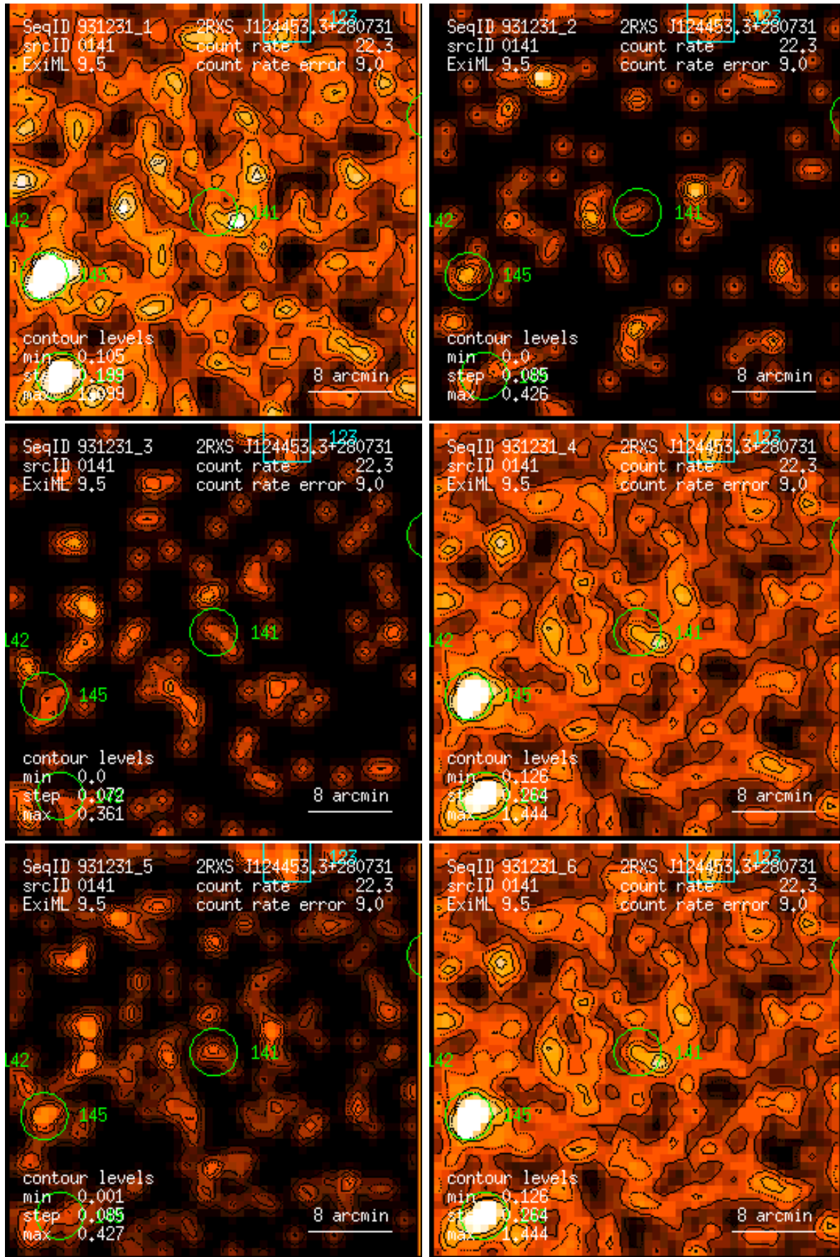
Figure 141: RASS 931231: detection 0141: band rate images, Gaussian filter: (1) PSPC channels 11 – 41, (2) 52 – 90, (3) 91 – 201, (4) 11 – 235, (5) 52 – 201, (6) 11 – 201. Broad band rates in counts/ks. Band rate contour levels in counts/ks/arcmin 2 .
