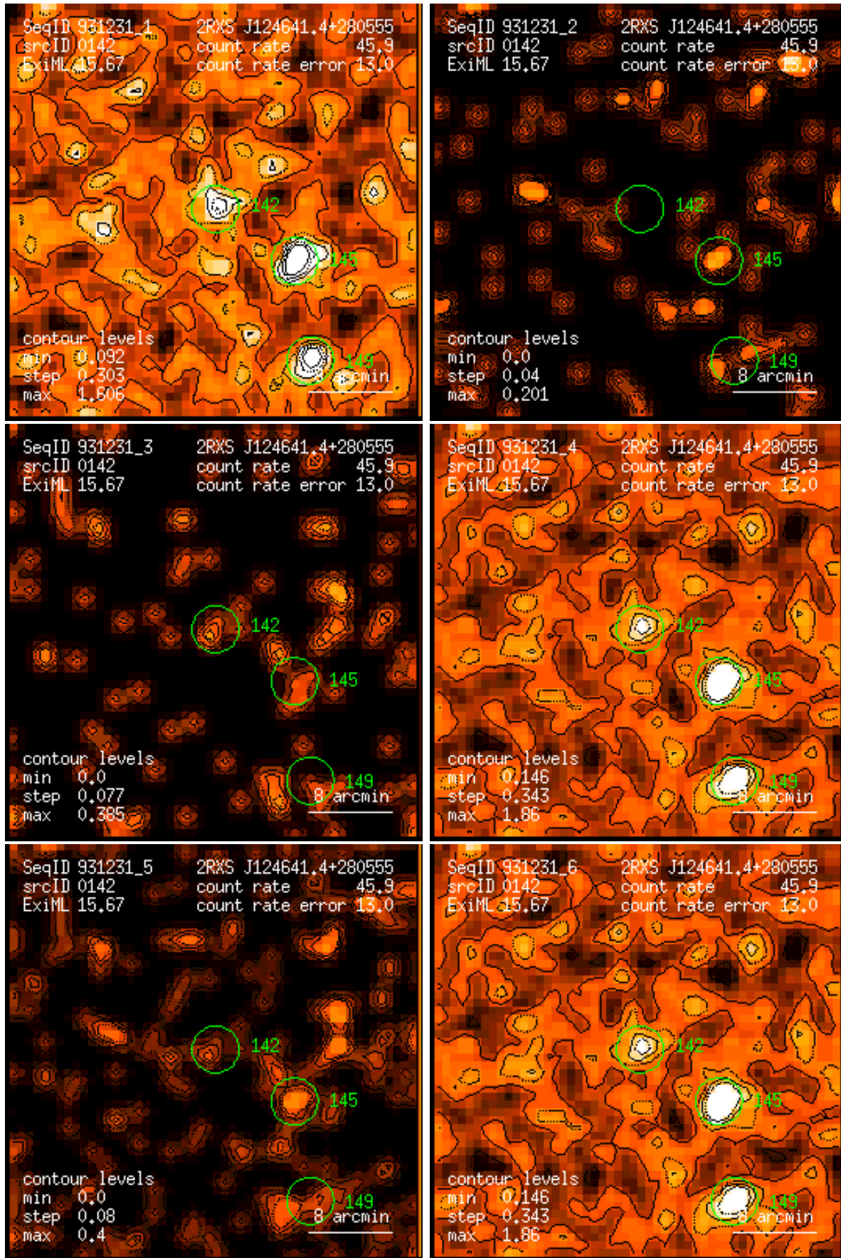
Figure 142: RASS 931231: detection 0142: band rate images, Gaussian filter: (1) PSPC channels 11 – 41, (2) 52 – 90, (3) 91 – 201, (4) 11 – 235, (5) 52 – 201, (6) 11 – 201. Broad band rates in counts/ks. Band rate contour levels in counts/ks/arcmin 2 .
