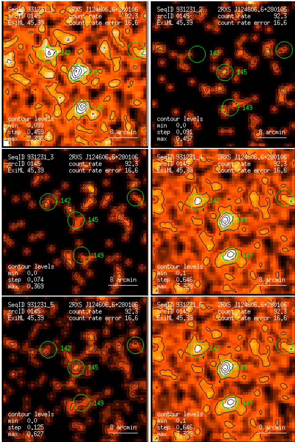
Figure 145: RASS 931231: detection 0145: band rate images, Gaussian filter: (1) PSPC channels 11 – 41, (2) 52 – 90, (3) 91 – 201, (4) 11 – 235, (5) 52 – 201, (6) 11 – 201. Broad band rates in counts/ks. Band rate contour levels in counts/ks/arcmin 2 .
