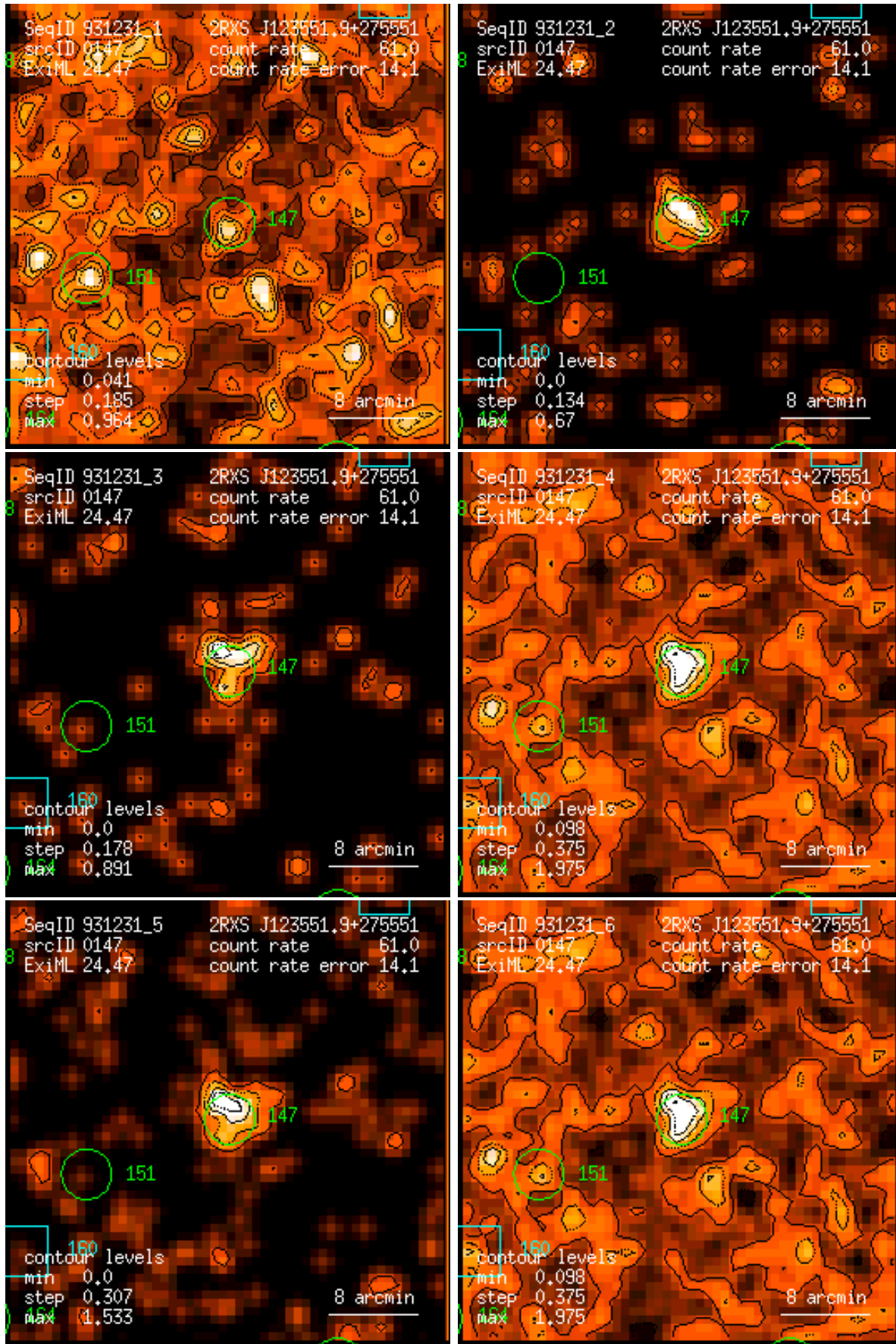
Figure 147: RASS 931231: detection 0147: band rate images, Gaussian filter: (1) PSPC channels 11 – 41, (2) 52 – 90, (3) 91 – 201, (4) 11 – 235, (5) 52 – 201, (6) 11 – 201. Broad band rates in counts/ks. Band rate contour levels in counts/ks/arcmin 2 .
