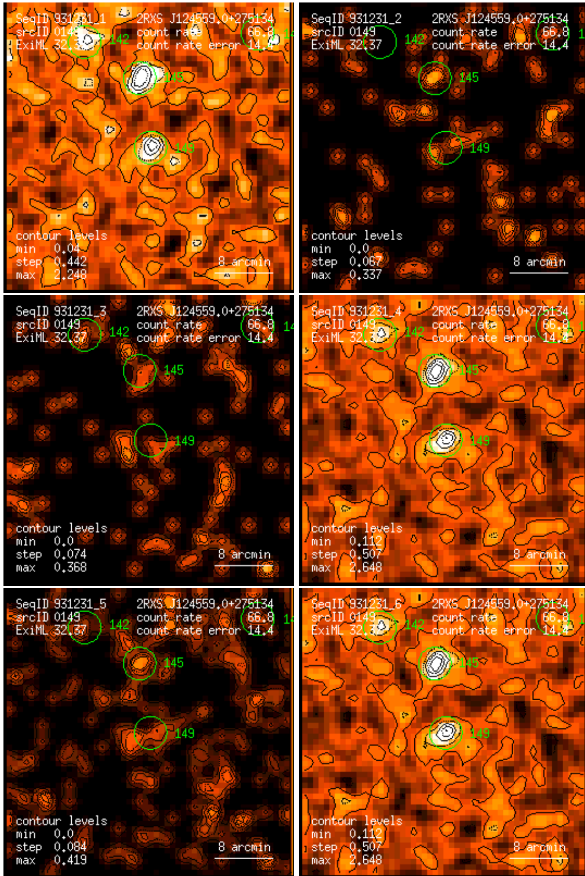
Figure 149: RASS 931231: detection 0149: band rate images, Gaussian filter: (1) PSPC channels 11 – 41, (2) 52 – 90, (3) 91 – 201, (4) 11 – 235, (5) 52 – 201, (6) 11 – 201. Broad band rates in counts/ks. Band rate contour levels in counts/ks/arcmin 2 .
