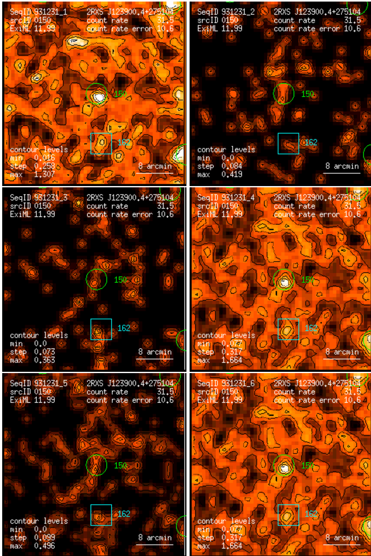
Figure 150: RASS 931231: detection 0150: band rate images, Gaussian filter: (1) PSPC channels 11 – 41, (2) 52 – 90, (3) 91 – 201, (4) 11 – 235, (5) 52 – 201, (6) 11 – 201. Broad band rates in counts/ks. Band rate contour levels in counts/ks/arcmin 2 .
