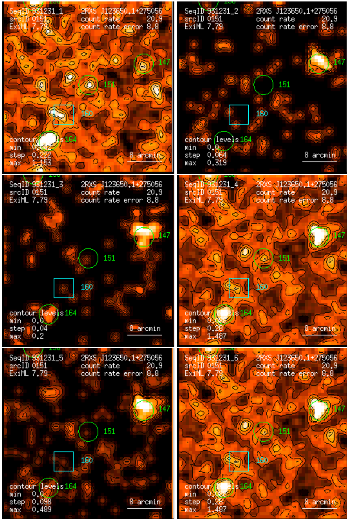
Figure 151: RASS 931231: detection 0151: band rate images, Gaussian filter: (1) PSPC channels 11 – 41, (2) 52 – 90, (3) 91 – 201, (4) 11 – 235, (5) 52 – 201, (6) 11 – 201. Broad band rates in counts/ks. Band rate contour levels in counts/ks/arcmin 2 .
