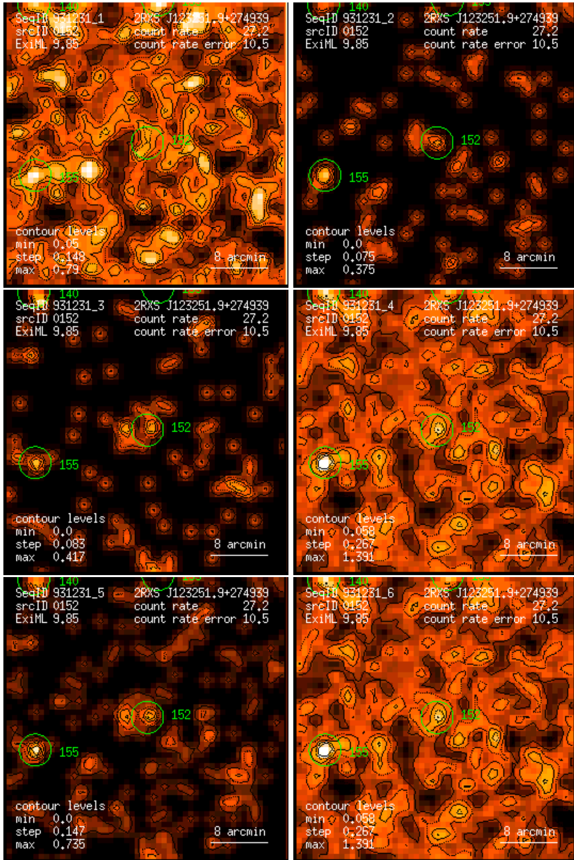
Figure 152: RASS 931231: detection 0152: band rate images, Gaussian filter: (1) PSPC channels 11 – 41, (2) 52 – 90, (3) 91 – 201, (4) 11 – 235, (5) 52 – 201, (6) 11 – 201. Broad band rates in counts/ks. Band rate contour levels in counts/ks/arcmin 2 .
