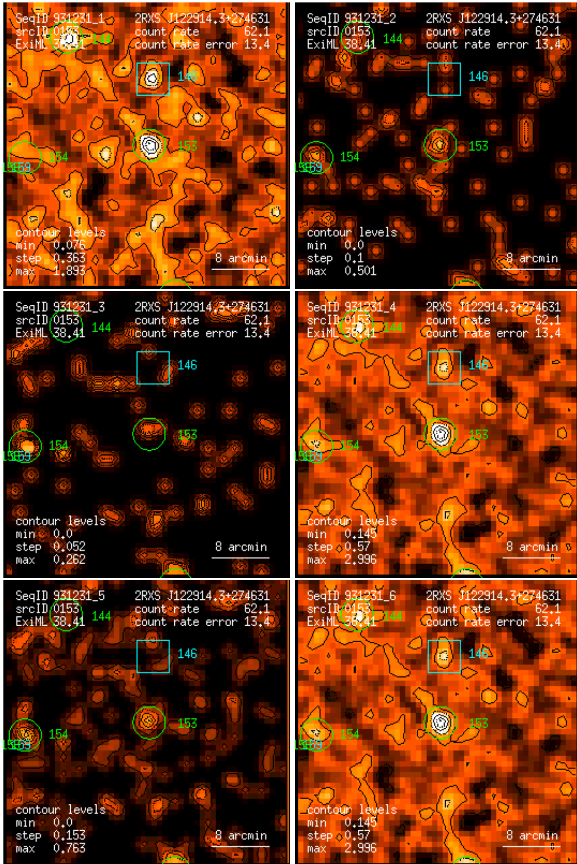
Figure 153: RASS 931231: detection 0153: band rate images, Gaussian filter: (1) PSPC channels 11 – 41, (2) 52 – 90, (3) 91 – 201, (4) 11 – 235, (5) 52 – 201, (6) 11 – 201. Broad band rates in counts/ks. Band rate contour levels in counts/ks/arcmin 2 .
