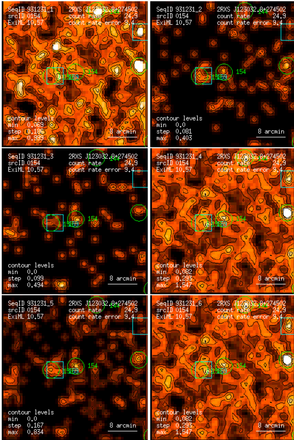
Figure 154: RASS 931231: detection 0154: band rate images, Gaussian filter: (1) PSPC channels 11 – 41, (2) 52 – 90, (3) 91 – 201, (4) 11 – 235, (5) 52 – 201, (6) 11 – 201. Broad band rates in counts/ks. Band rate contour levels in counts/ks/arcmin 2 .
