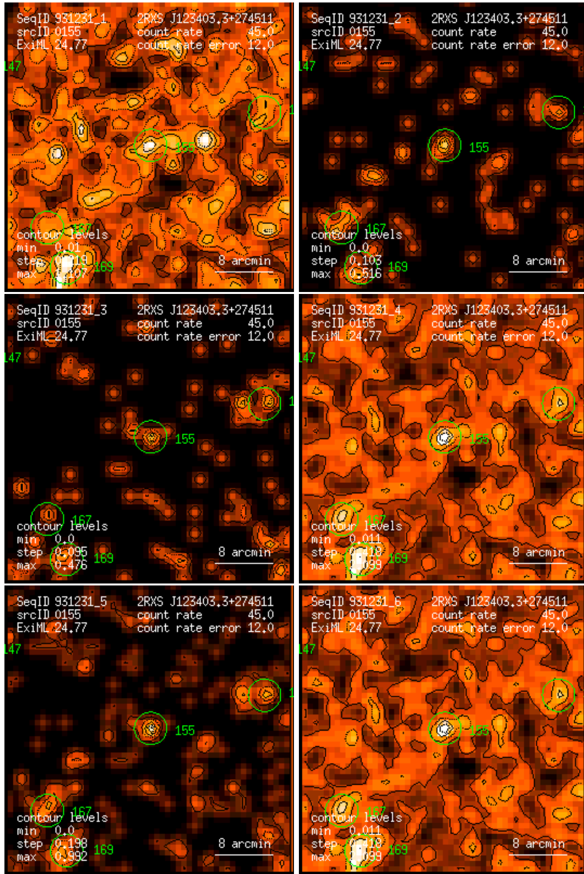
Figure 155: RASS 931231: detection 0155: band rate images, Gaussian filter: (1) PSPC channels 11 – 41, (2) 52 – 90, (3) 91 – 201, (4) 11 – 235, (5) 52 – 201, (6) 11 – 201. Broad band rates in counts/ks. Band rate contour levels in counts/ks/arcmin 2 .
