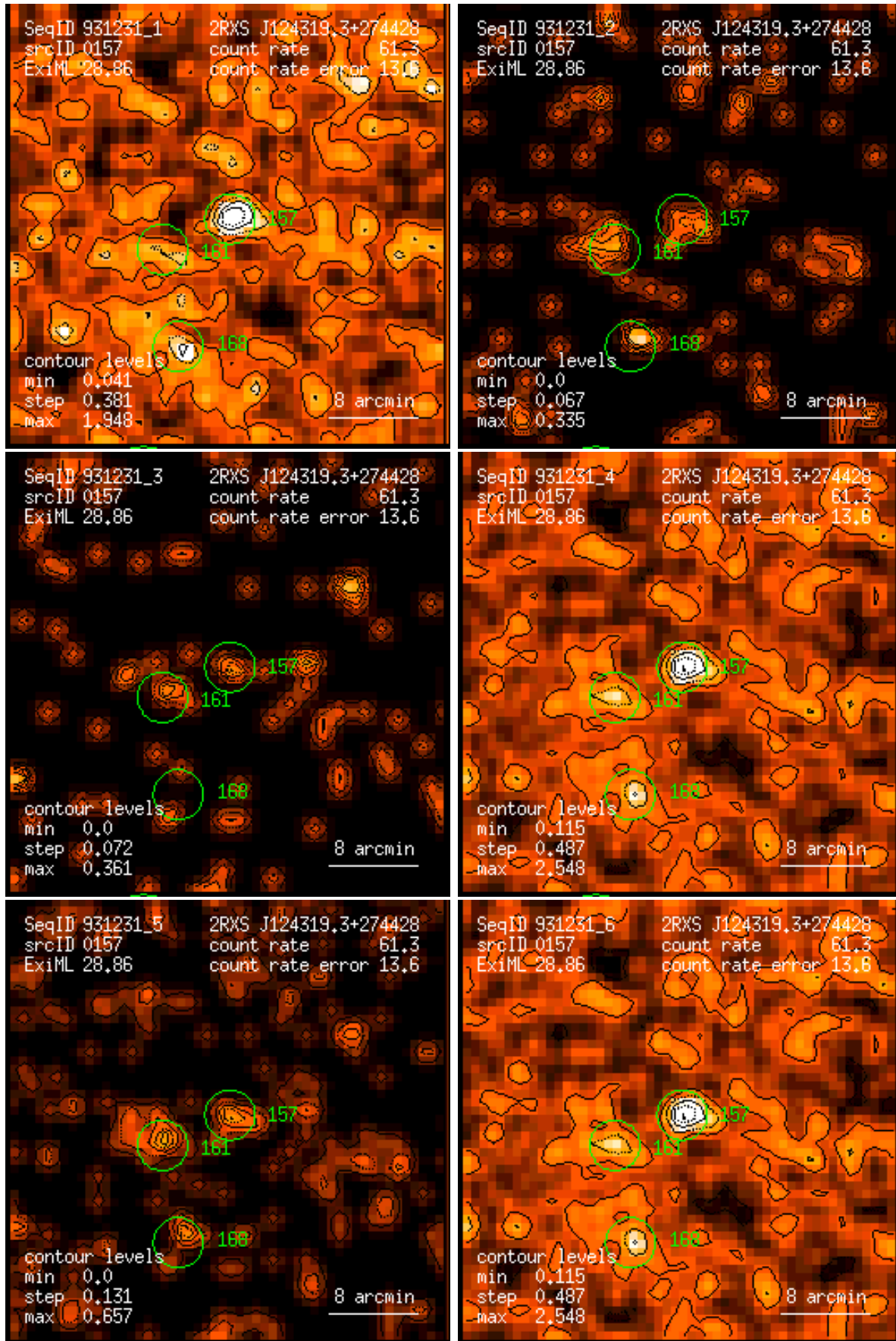
Figure 157: RASS 931231: detection 0157: band rate images, Gaussian filter: (1) PSPC channels 11 – 41, (2) 52 – 90, (3) 91 – 201, (4) 11 – 235, (5) 52 – 201, (6) 11 – 201. Broad band rates in counts/ks. Band rate contour levels in counts/ks/arcmin 2 .
