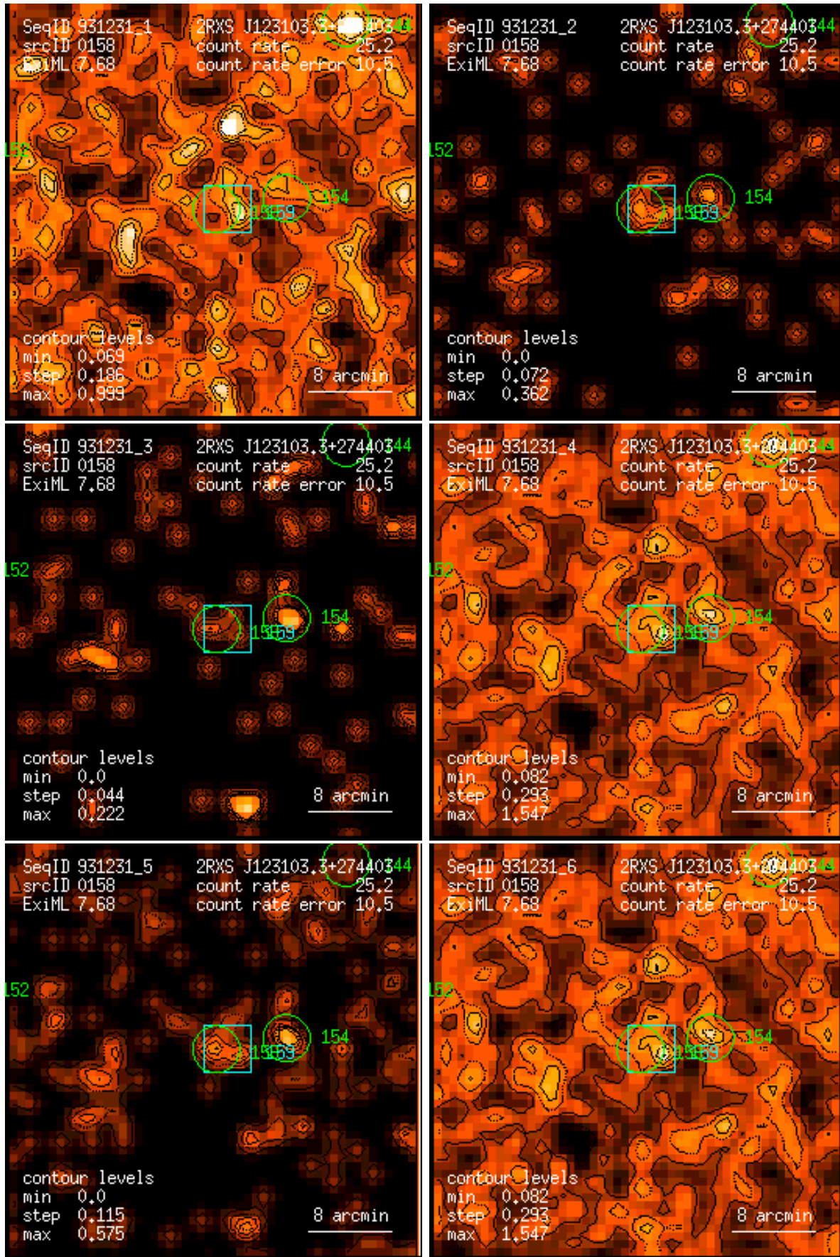
Figure 158: RASS 931231: detection 0158: band rate images, Gaussian filter: (1) PSPC channels 11 – 41, (2) 52 – 90, (3) 91 – 201, (4) 11 – 235, (5) 52 – 201, (6) 11 – 201. Broad band rates in counts/ks. Band rate contour levels in counts/ks/arcmin 2 .
