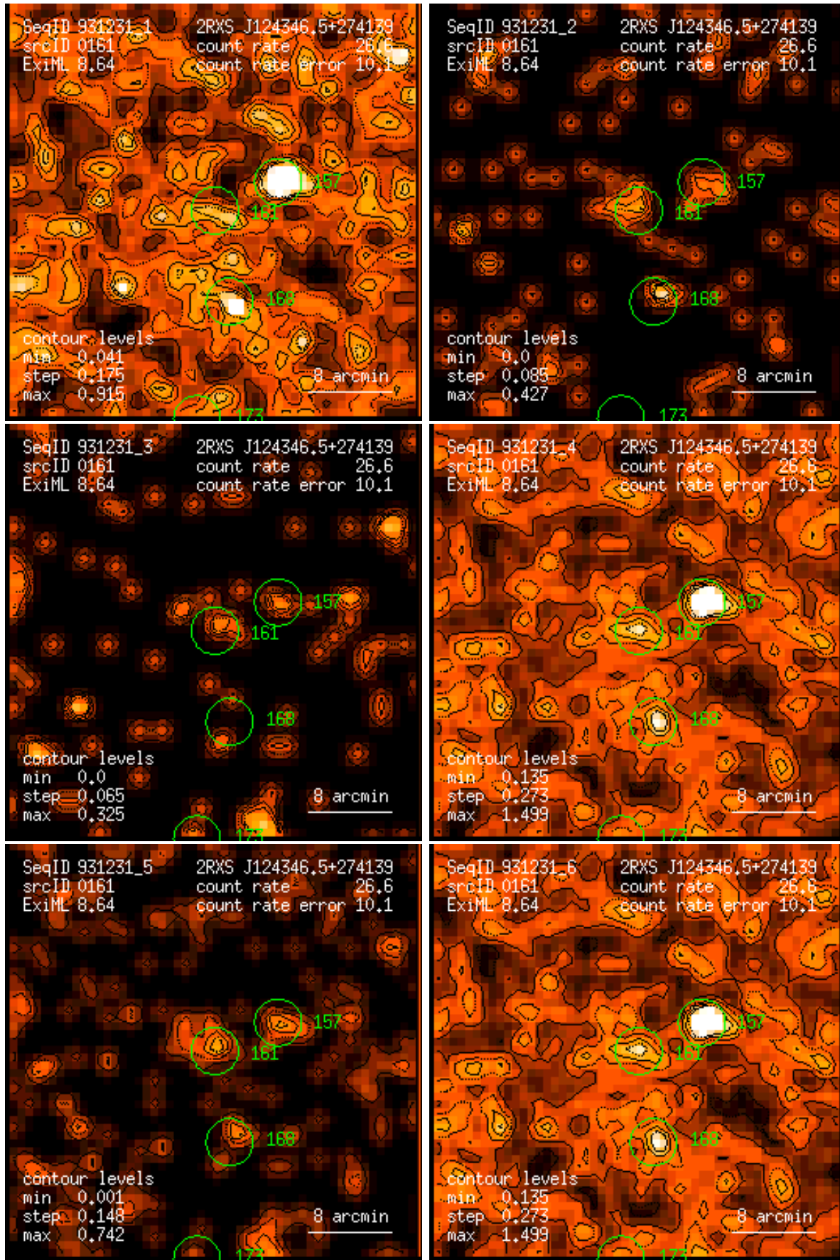
Figure 161: RASS 931231: detection 0161: band rate images, Gaussian filter: (1) PSPC channels 11 – 41, (2) 52 – 90, (3) 91 – 201, (4) 11 – 235, (5) 52 – 201, (6) 11 – 201. Broad band rates in counts/ks. Band rate contour levels in counts/ks/arcmin 2 .
