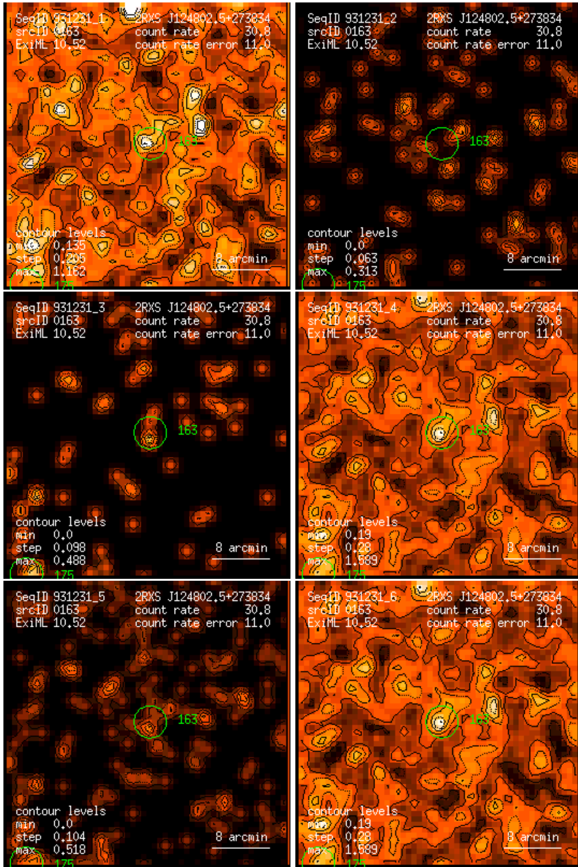
Figure 163: RASS 931231: detection 0163: band rate images, Gaussian filter: (1) PSPC channels 11 – 41, (2) 52 – 90, (3) 91 – 201, (4) 11 – 235, (5) 52 – 201, (6) 11 – 201. Broad band rates in counts/ks. Band rate contour levels in counts/ks/arcmin 2 .
