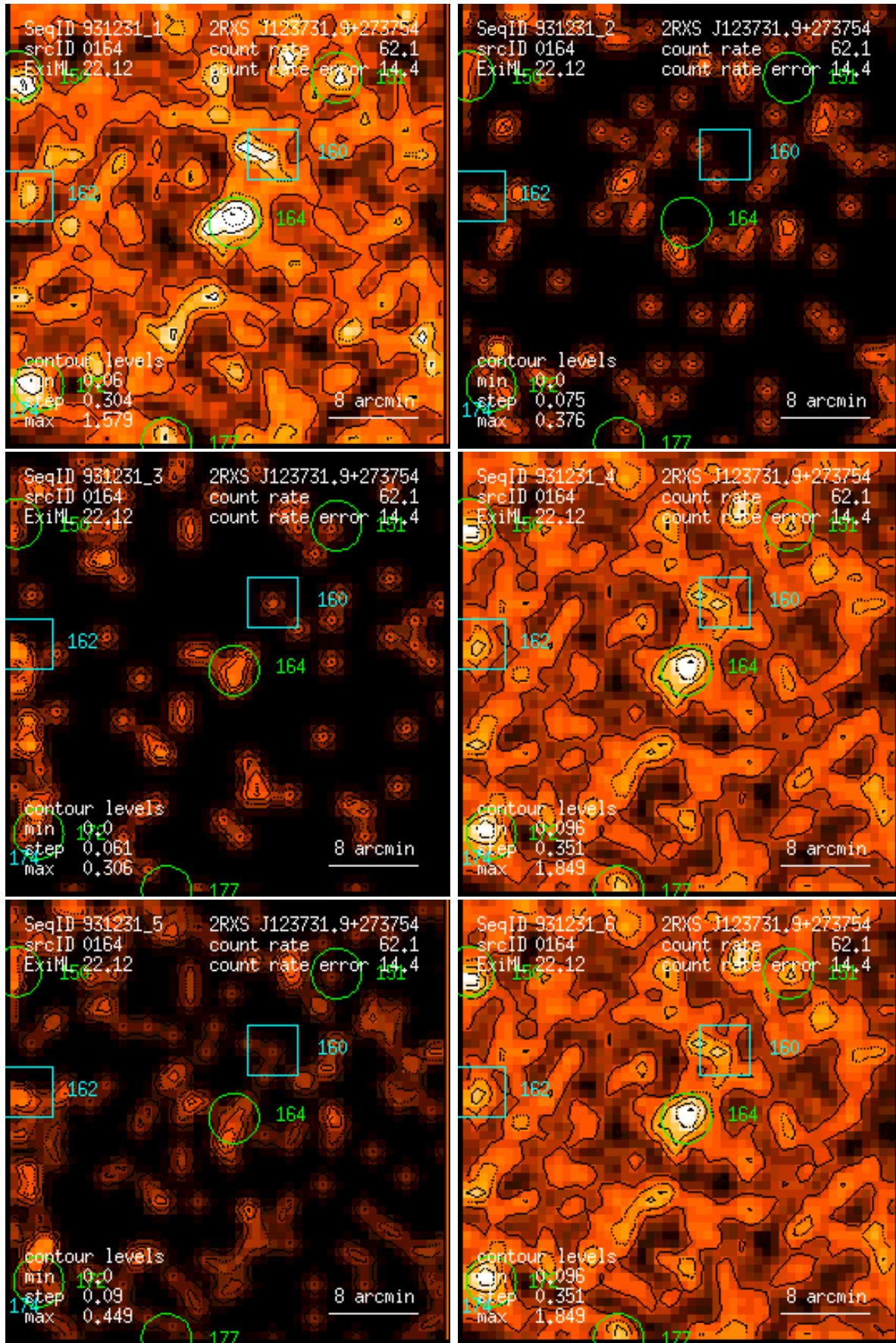
Figure 164: RASS 931231: detection 0164: band rate images, Gaussian filter: (1) PSPC channels 11 – 41, (2) 52 – 90, (3) 91 – 201, (4) 11 – 235, (5) 52 – 201, (6) 11 – 201. Broad band rates in counts/ks. Band rate contour levels in counts/ks/arcmin 2 .
