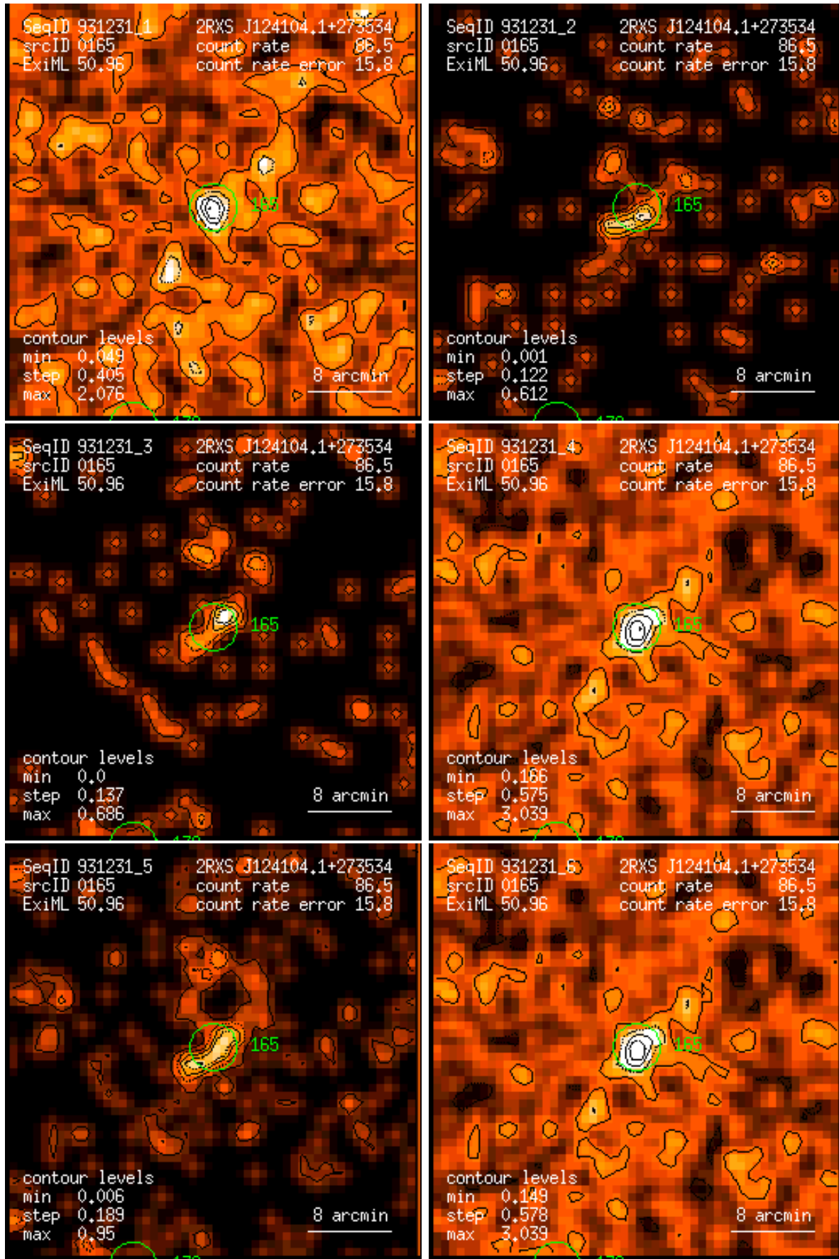
Figure 165: RASS 931231: detection 0165: band rate images, Gaussian filter: (1) PSPC channels 11 – 41, (2) 52 – 90, (3) 91 – 201, (4) 11 – 235, (5) 52 – 201, (6) 11 – 201. Broad band rates in counts/ks. Band rate contour levels in counts/ks/arcmin 2 .
