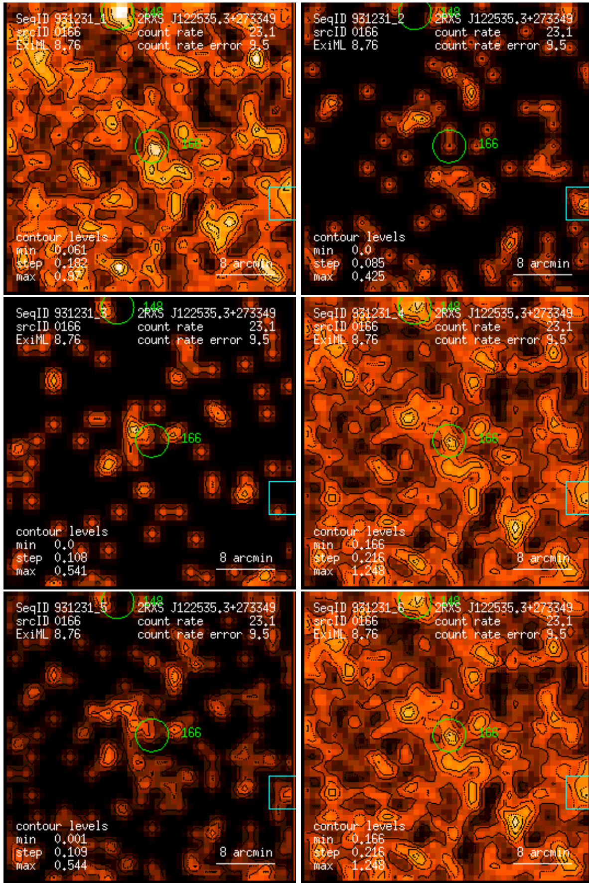
Figure 166: RASS 931231: detection 0166: band rate images, Gaussian filter: (1) PSPPC channels 11 – 41, (2) 52 – 90, (3) 91 – 201, (4) 11 – 235, (5) 52 – 201, (6) 11 – 201. Broad band rates in counts/ks. Band rate contour levels in counts/ks/arcmin 2 .
