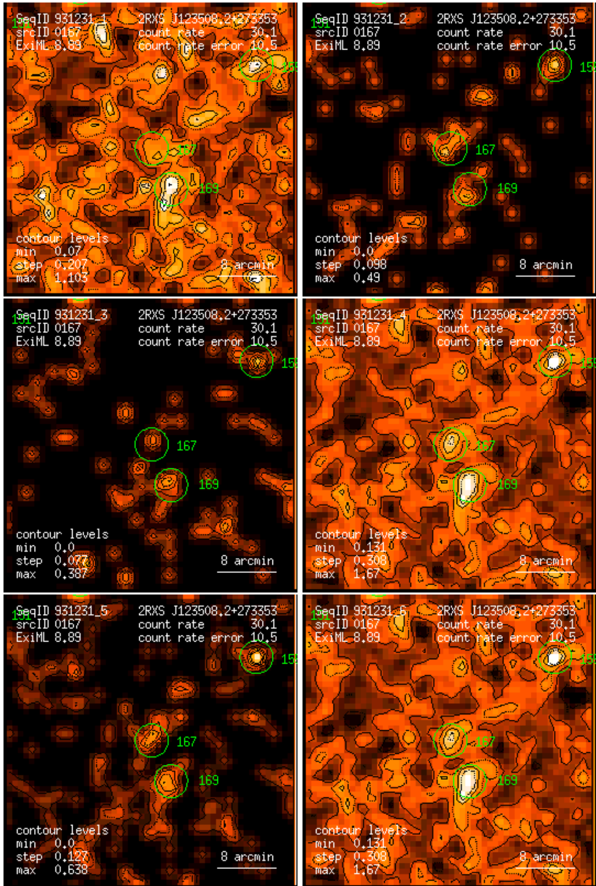
Figure 167: RASS 931231: detection 0167: band rate images, Gaussian filter: (1) PSPC channels 11 – 41, (2) 52 – 90, (3) 91 – 201, (4) 11 – 235, (5) 52 – 201, (6) 11 – 201. Broad band rates in counts/ks. Band rate contour levels in counts/ks/arcmin 2 .
