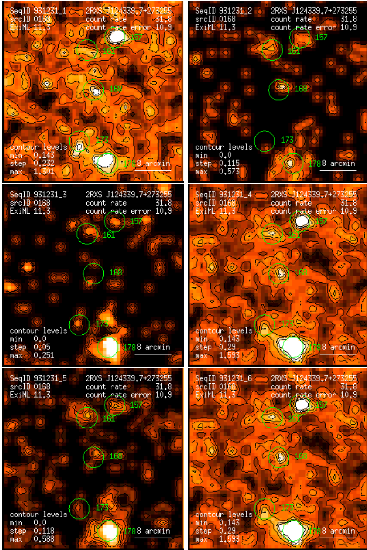
Figure 168: RASS 931231: detection 0168: band rate images, Gaussian filter: (1) PSPC channels 11 – 41, (2) 52 – 90, (3) 91 – 201, (4) 11 – 235, (5) 52 – 201, (6) 11 – 201. Broad band rates in counts/ks. Band rate contour levels in counts/ks/arcmin 2 .
