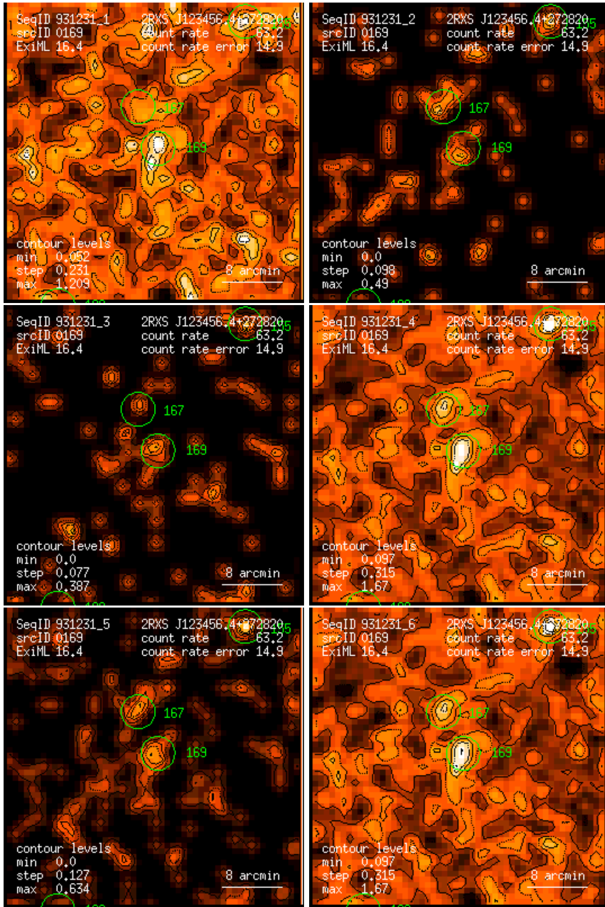
Figure 169: RASS 931231: detection 0169: band rate images, Gaussian filter: (1) PSPC channels 11 – 41, (2) 52 – 90, (3) 91 – 201, (4) 11 – 235, (5) 52 – 201, (6) 11 – 201. Broad band rates in counts/ks. Band rate contour levels in counts/ks/arcmin 2 .
