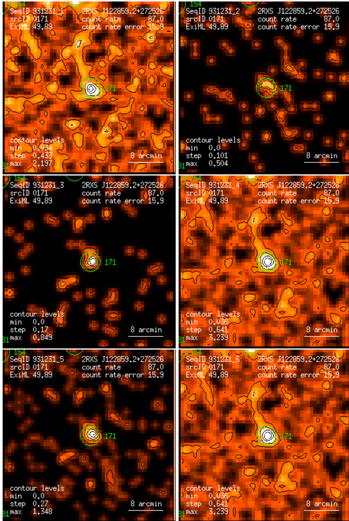
Figure 171: RASS 931231: detection 0171: band rate images, Gaussian filter: (1) PSPC channels 11 – 41, (2) 52 – 90, (3) 91 – 201, (4) 11 – 235, (5) 52 – 201, (6) 11 – 201. Broad band rates in counts/ks. Band rate contour levels in counts/ks/arcmin 2 .
