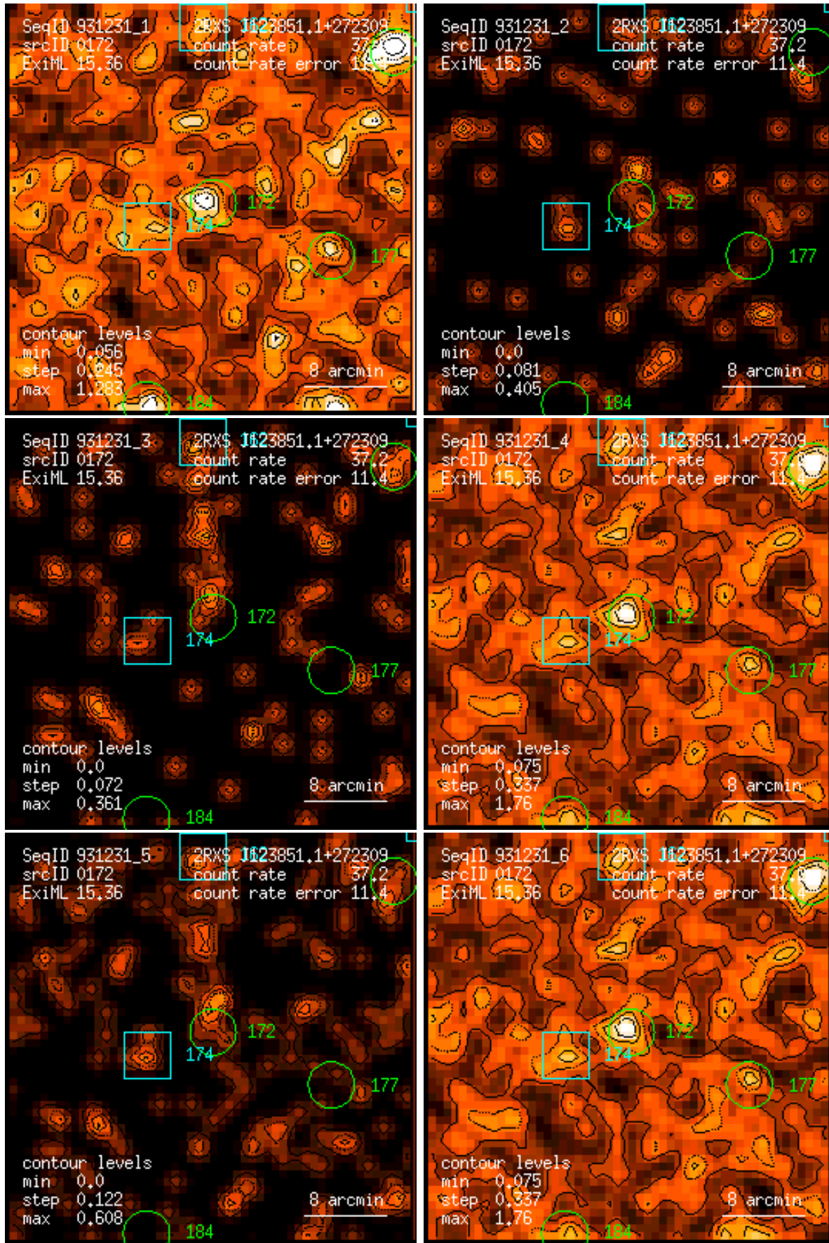
Figure 172: RASS 931231: detection 0172: band rate images, Gaussian filter: (1) PSPC channels 11 – 41, (2) 52 – 90, (3) 91 – 201, (4) 11 – 235, (5) 52 – 201, (6) 11 – 201. Broad band rates in counts/ks. Band rate contour levels in counts/ks/arcmin 2 .
